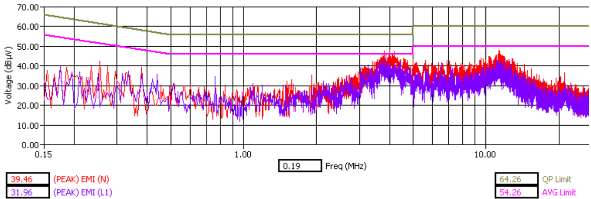
WLAN Channel 1 - Tx Mode - Peak Detector
