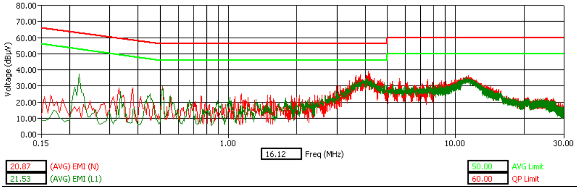
WLAN Channel 1 - Tx Mode - AVG Detector
