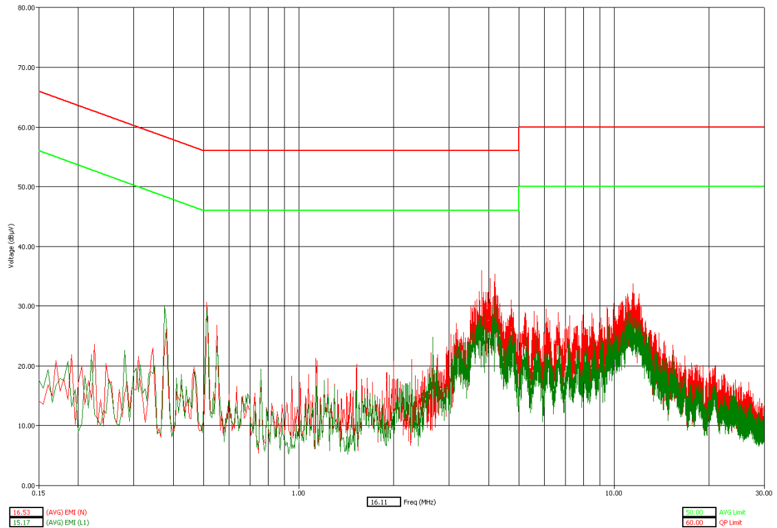
Bluetooth – Hopping - Tx Mode – AVG Detector
