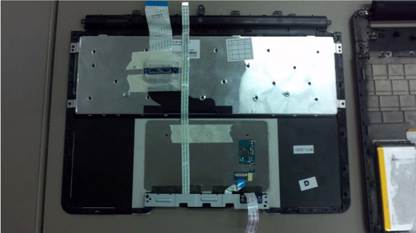
Photograph 5: Underside View of Keypad and Touchpad.
