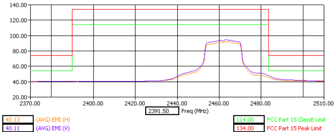
High Band Edge Y Orientation AVG Detector
