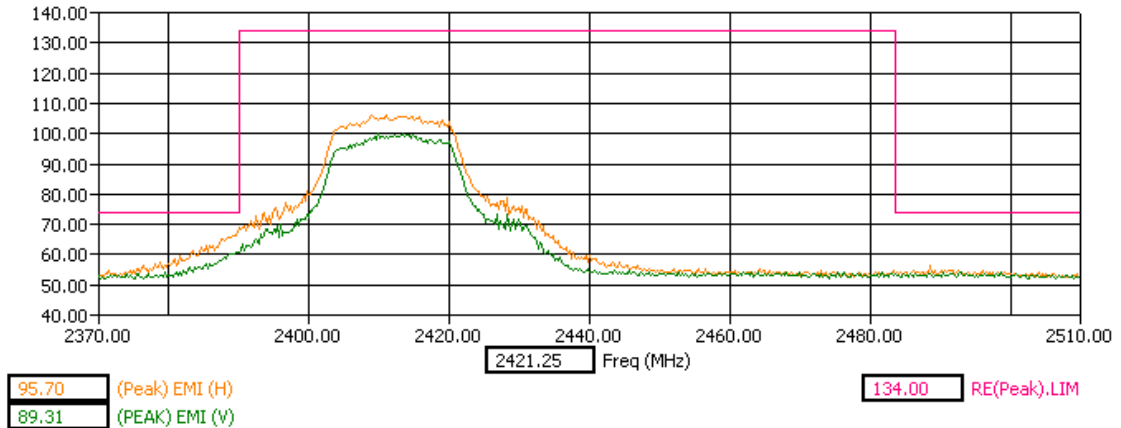
Low Band Edge Y Orientation Peak Detector
