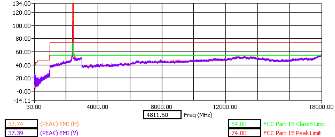
30 - 18000MHz Low Channel Dual Polarization Y
