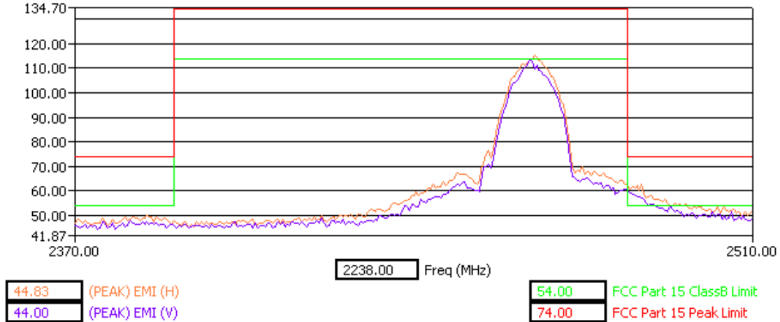
High Band Edge Y Orientation Peak Detector
