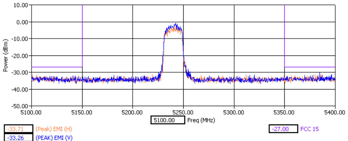
High Band Edge Z Orientation Peak Detector
