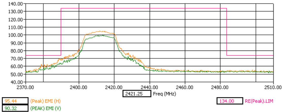
Low Band Edge Y Orientation Peak Detector
