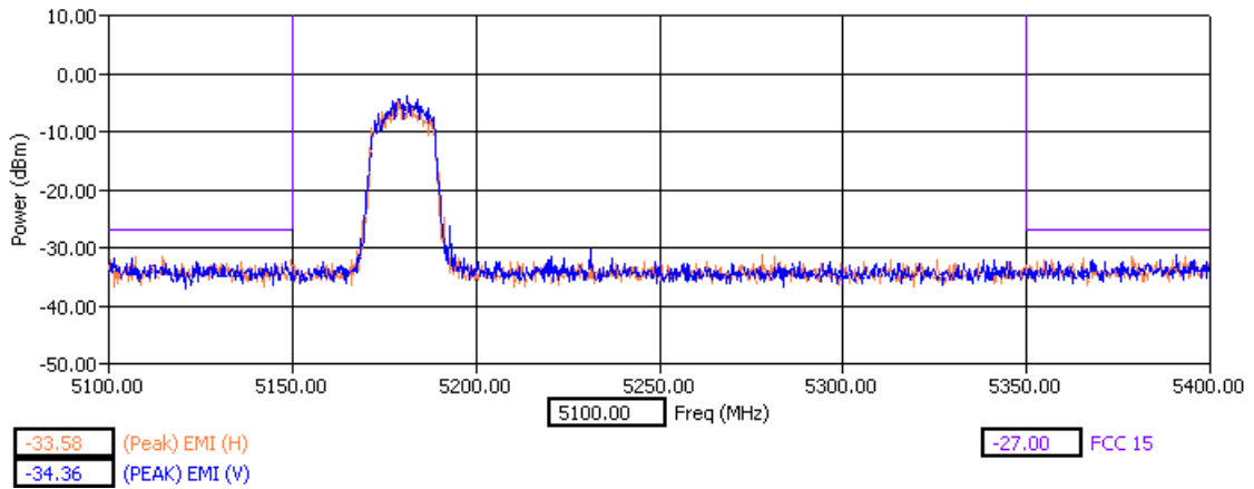
Low Band Edge Z Orientation Peak Detector
