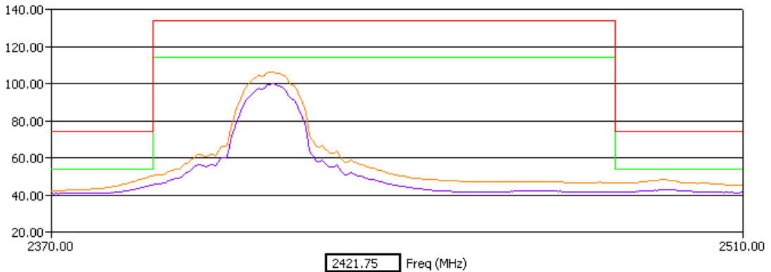
Low Band Edge Y Orientation AVG Detector
