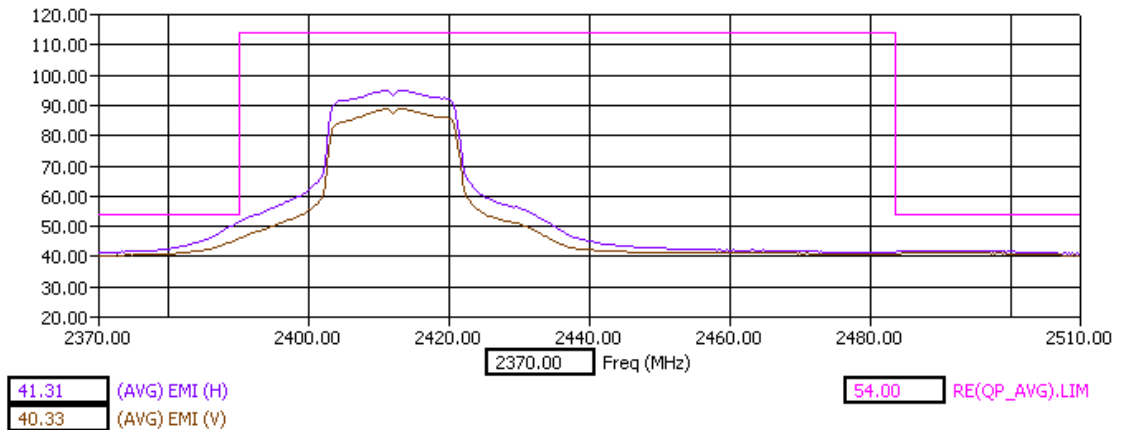
Low Band Edge Y Orientation AVG Detector
