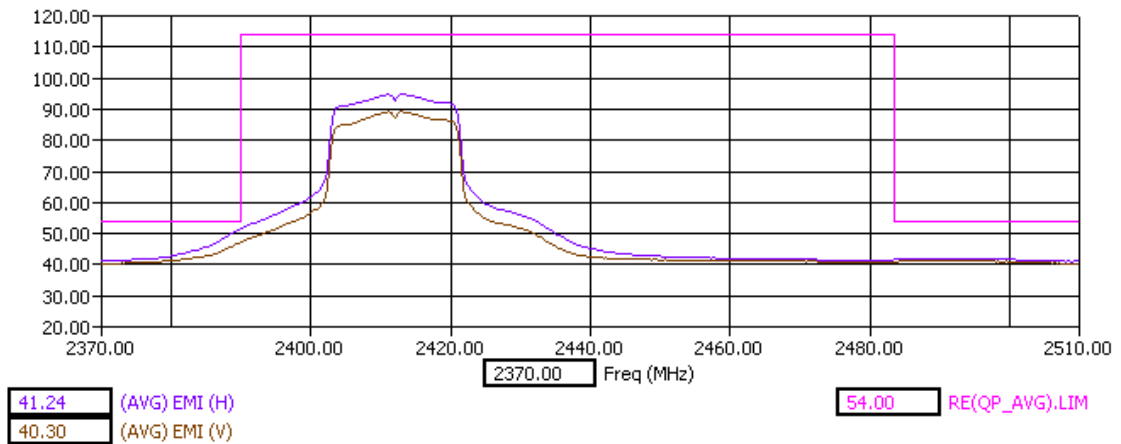
Low Band Edge Y Orientation AVG Detector
