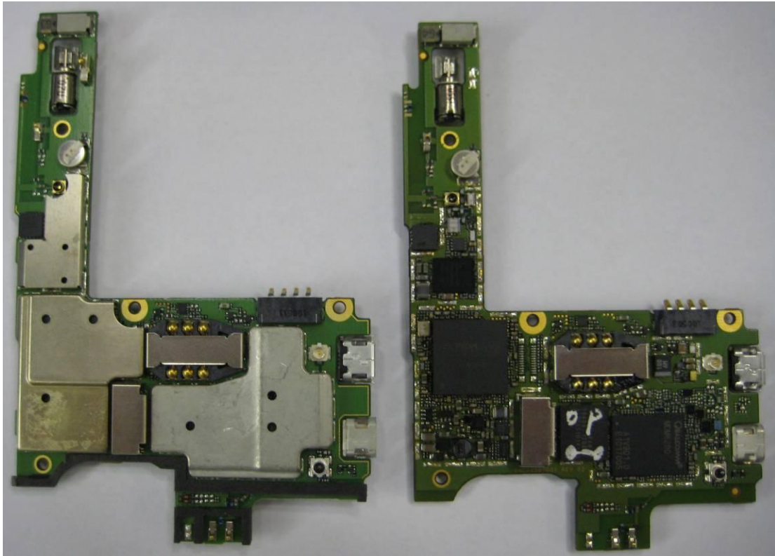
BOTTOM SIDE WITHOUT SHIELD
