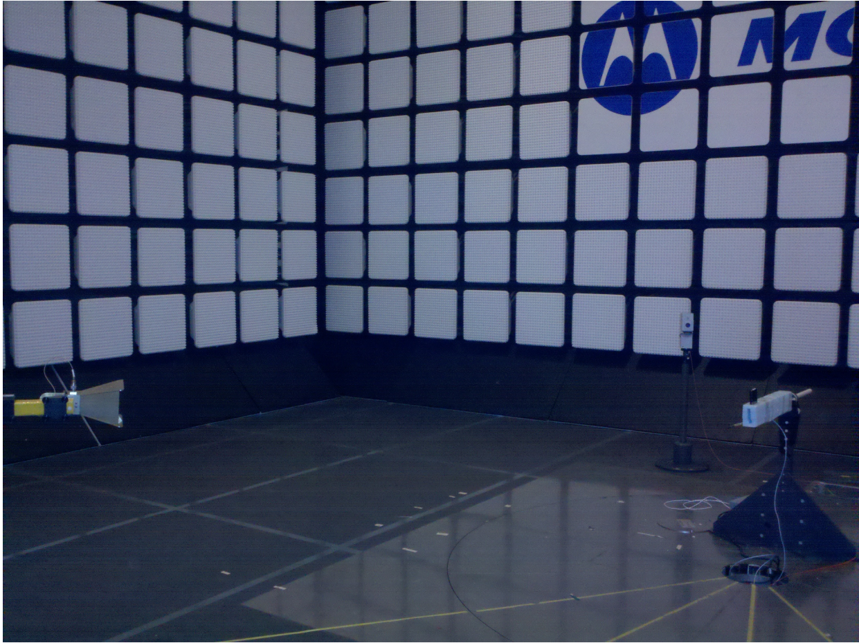
Radiated Emissions for Bluetooth & WLAN
