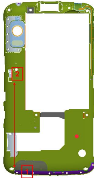
Figure 2: Antenna Separation Distances
