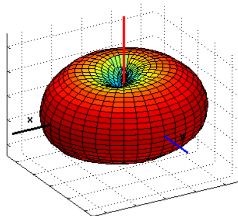
Figure 6a.6-4 Antenna pattern (Flip Closed).
