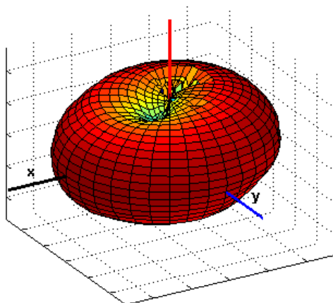
Figure 6a.6-3 Antenna pattern (Flip Open).
