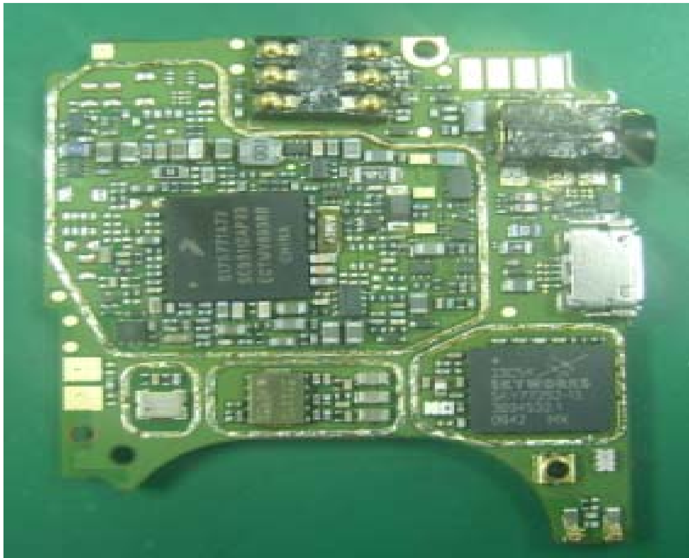
Photograph 9-4: Back side view of radio PC Board (Shields Removed).
