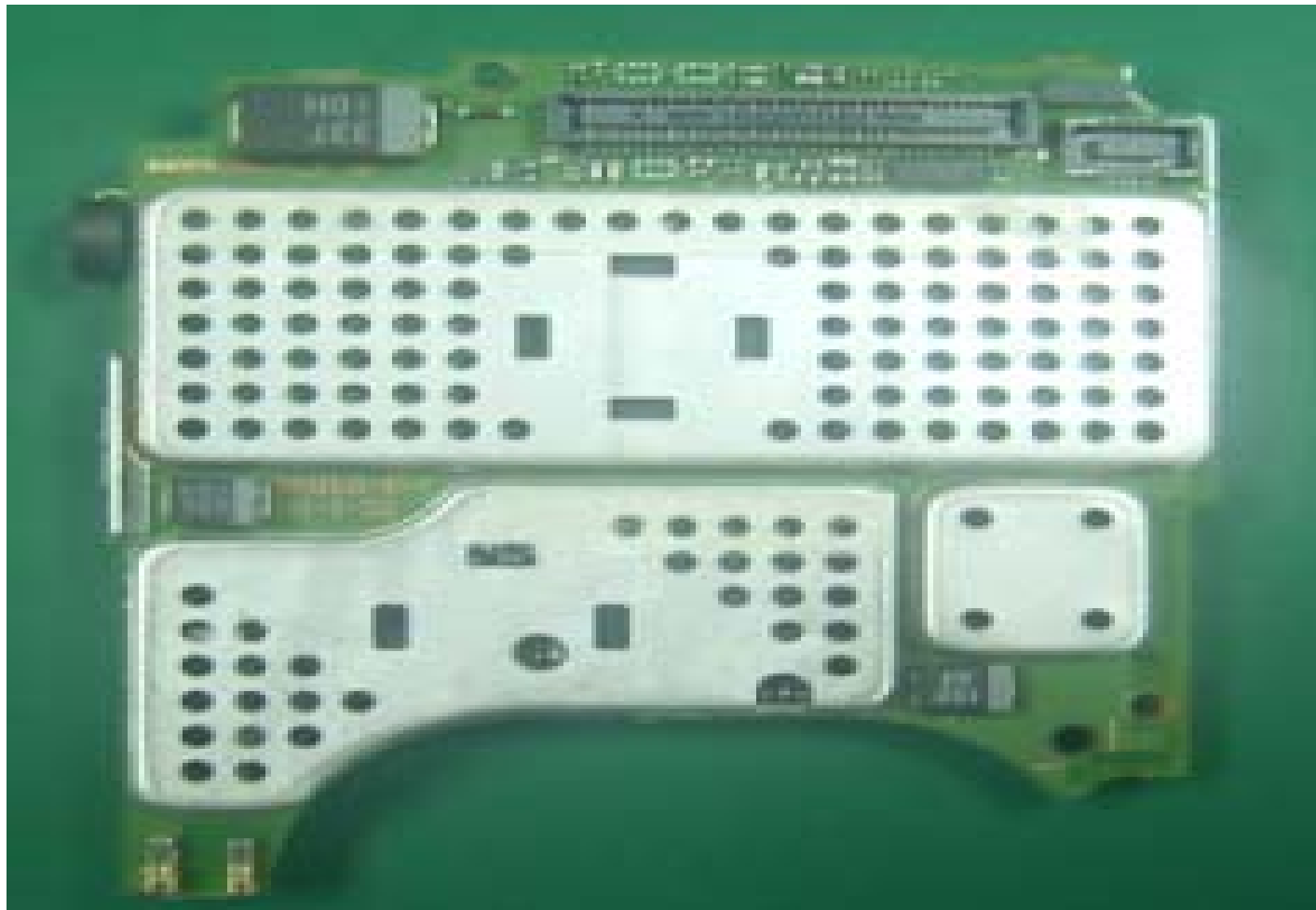
Photograph 9-1: Front side view of radio product PC Board.
