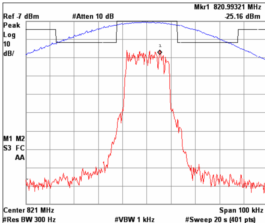
Figure 6a.2.1-12. iDEN 800 MHz Band, Quad-64QAM, Minimum Power, EA Emission Mask
