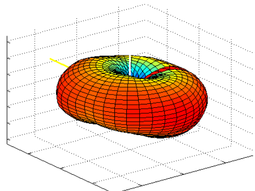
Figure 6a.6-6 Antenna pattern in the 900 MHz NBPCS frequency band (Flip Closed).
