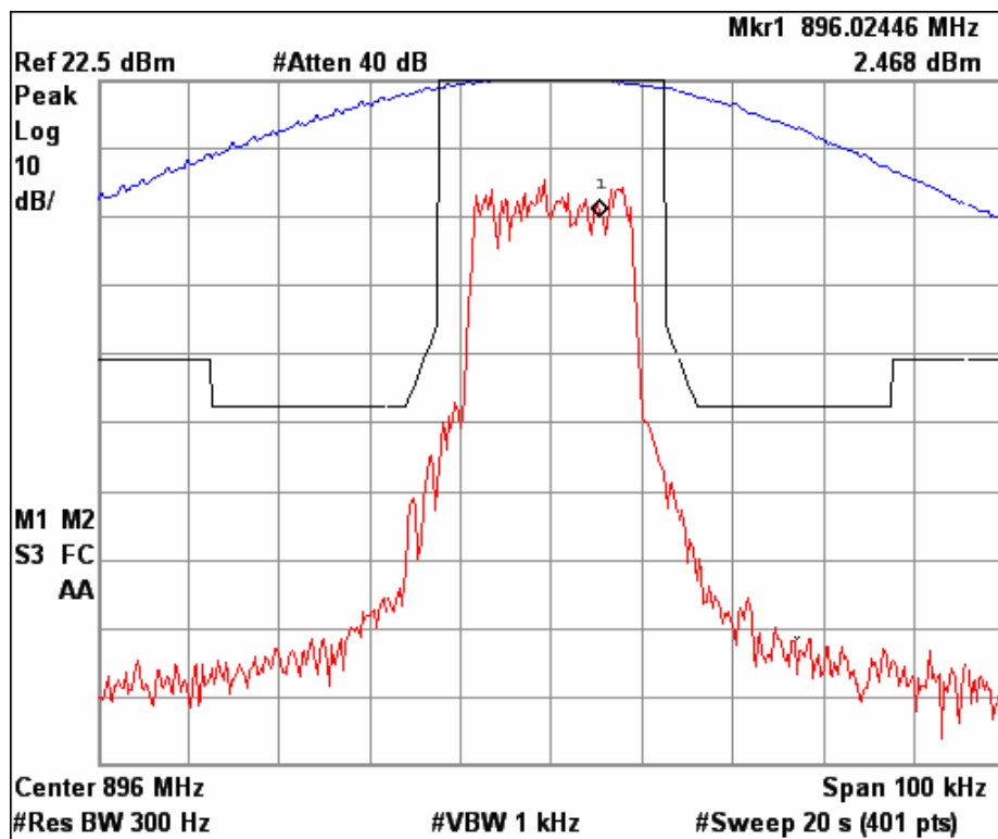
Figure 6a.2.2-7. iDEN 900 MHz Band, Quad-16QAM, Maximum Power, EA Emission Mask
