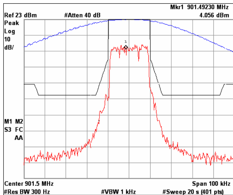
Figure 6b.2.1-1 iDEN NBPCS Band, Occupied Bandwidth, Quad-QPSK, Maximum Power.
