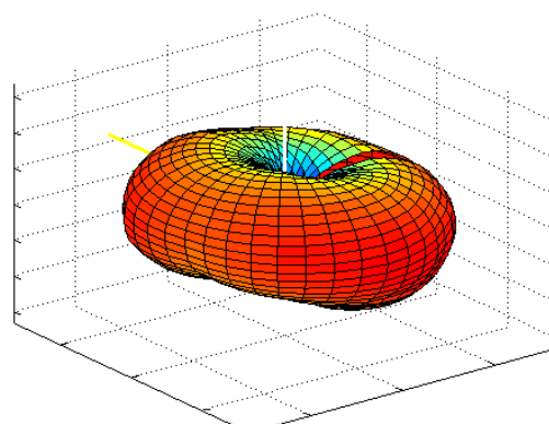
Figure 6a.6-3 Antenna pattern in the 900 MHz SMR frequency band (Flip Closed).
