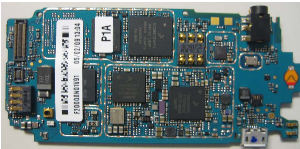
Photograph 9-2: Component side view of radio product PC Board, Shields removed.
