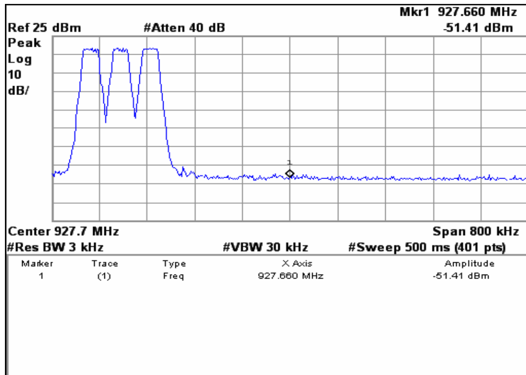
Figure 6b.2.2.8. Out-of-band transmitter spurious emissions high band edge, with hopping function enabled.
