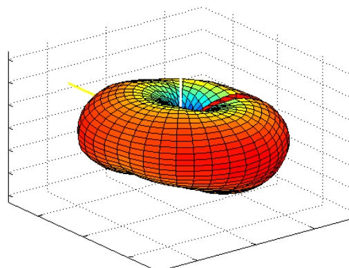
Figure 6b.5-2 Antenna pattern in the 800 MHz SMR frequency band (Flip Closed).
