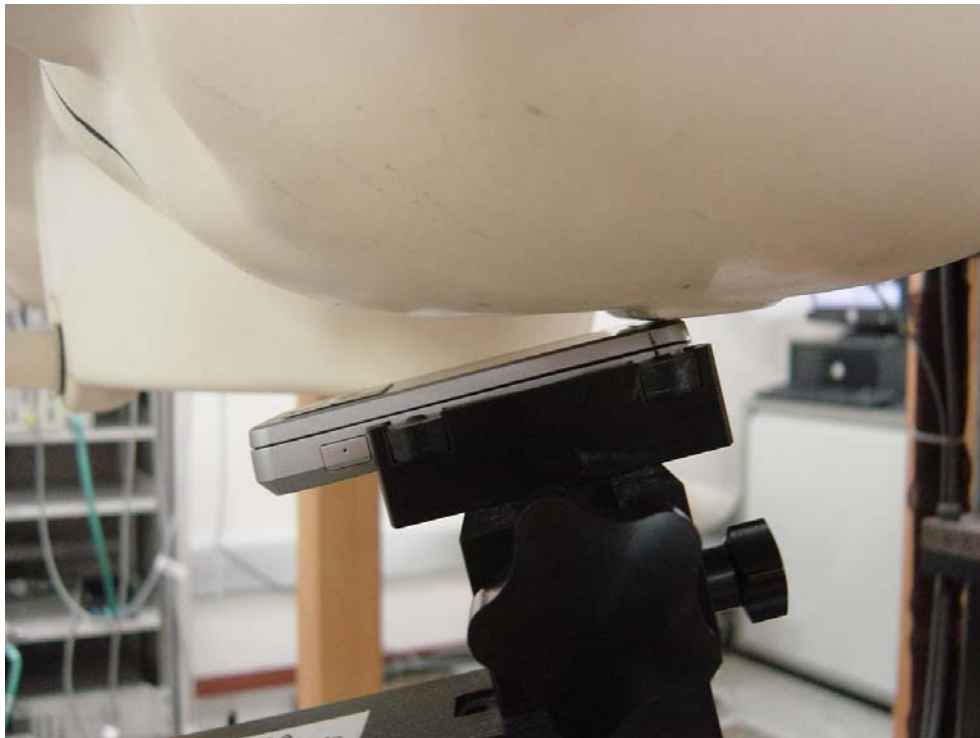
Figure 7: Phone Against the Head Phantom (15° Tilt – Slider Closed)
