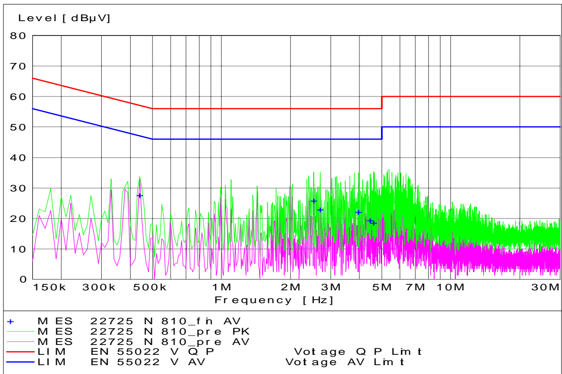
Channel 810 - Tx Mode PCS - Neutral Coupling
