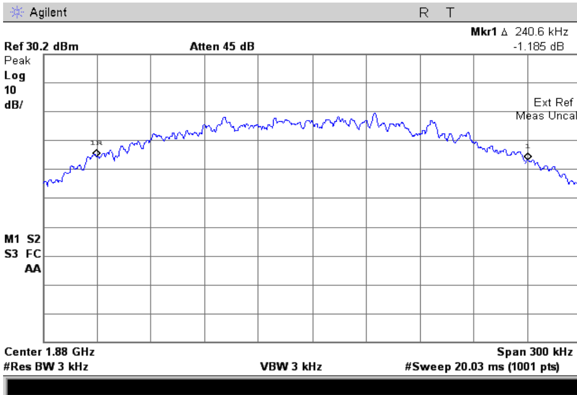
GSM 1900 – Occupied Bandwidth – Channel 661 (1880.00MHz)
