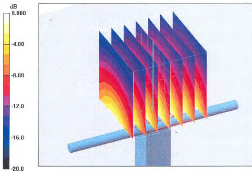
0 dB = 11.8mW/g
