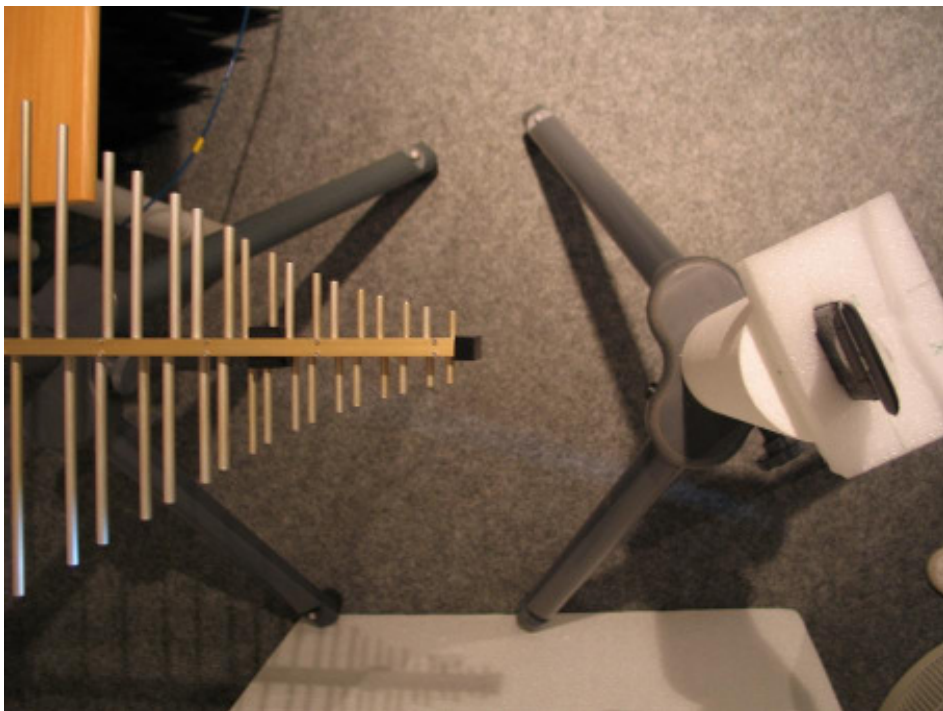
22235-1, IHDP56JF1 check for maximum radiation at position Z - Open
