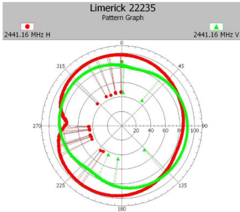
22235-1, IHDP56JF1 maximum radiation pattern position Z - Open
