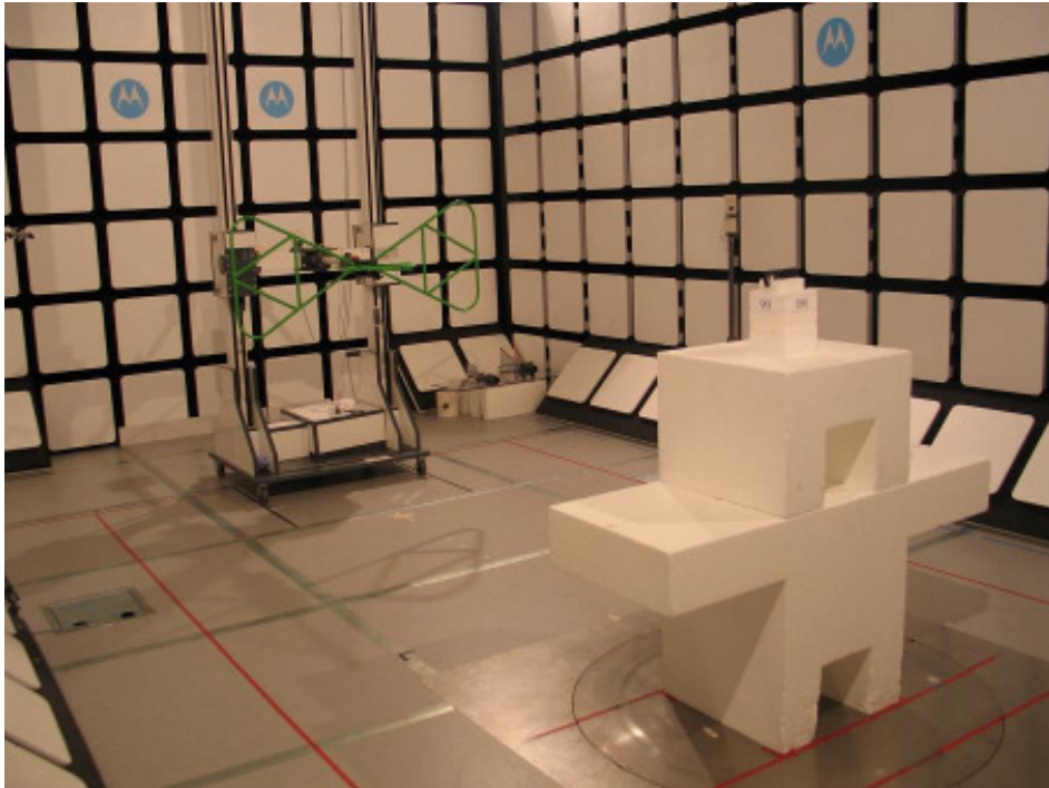
22235-1, IHDP56JF1 setup in semi-anechoic chamber – left side
