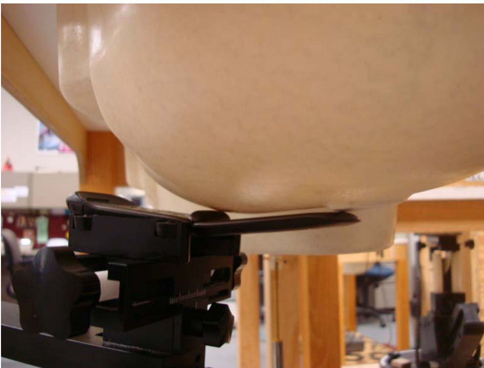
Figure 4. Transceiver against head, Cheek Touch position
