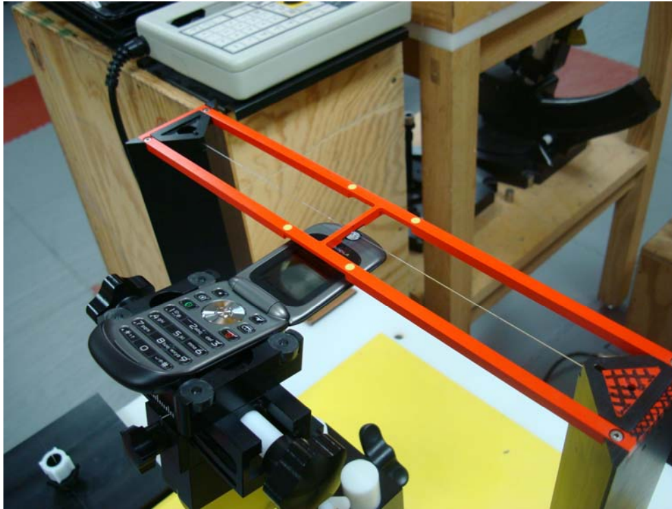
Figure 5. Positioning for RF Emissions
