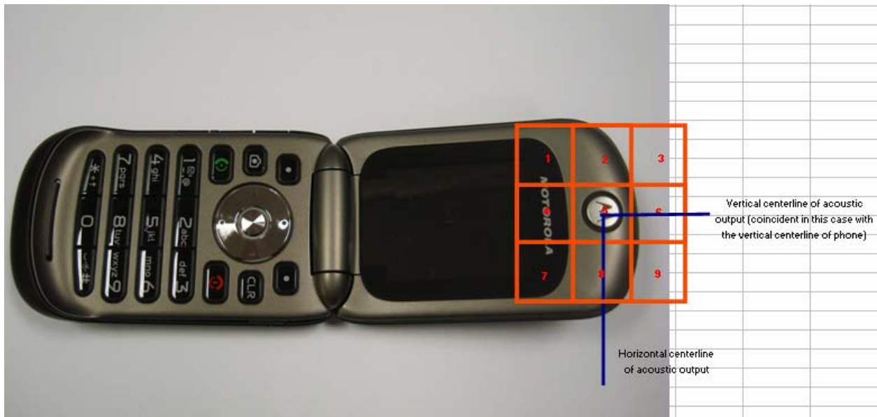
Figure 4. Phone Open - Orientation and Measurement Plane for RF Emissions Testing
