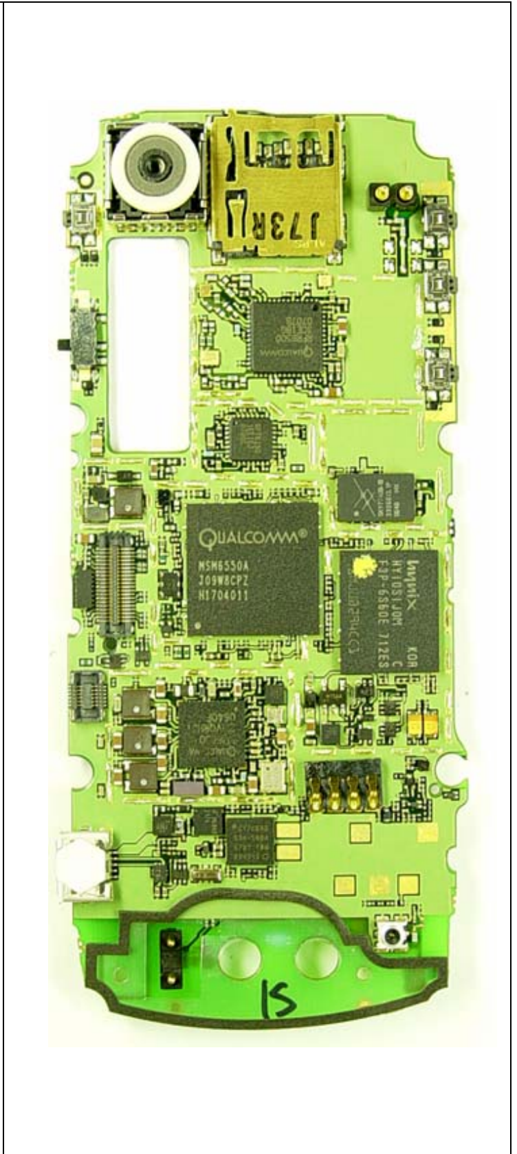
Main Board Top without Shieldcans
