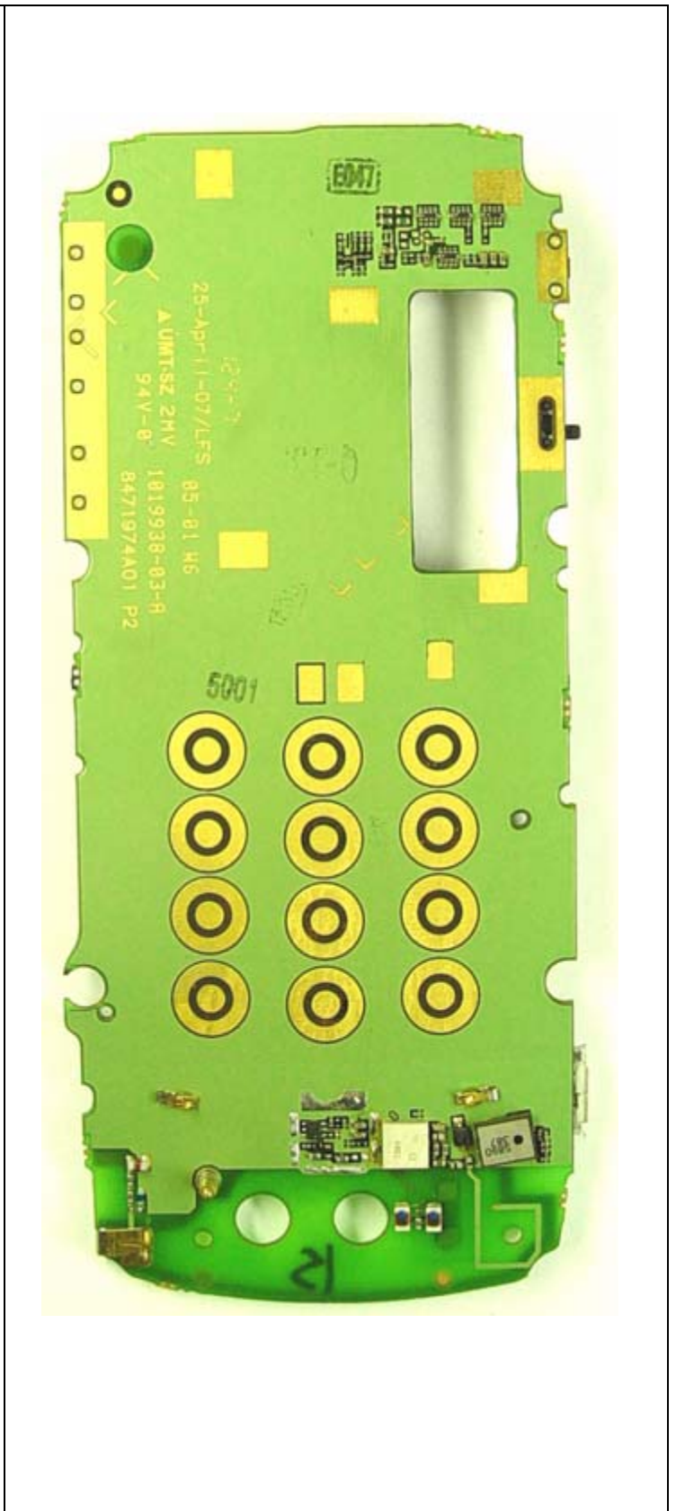
Main Board Bottom without Shieldcans & Domesheet
