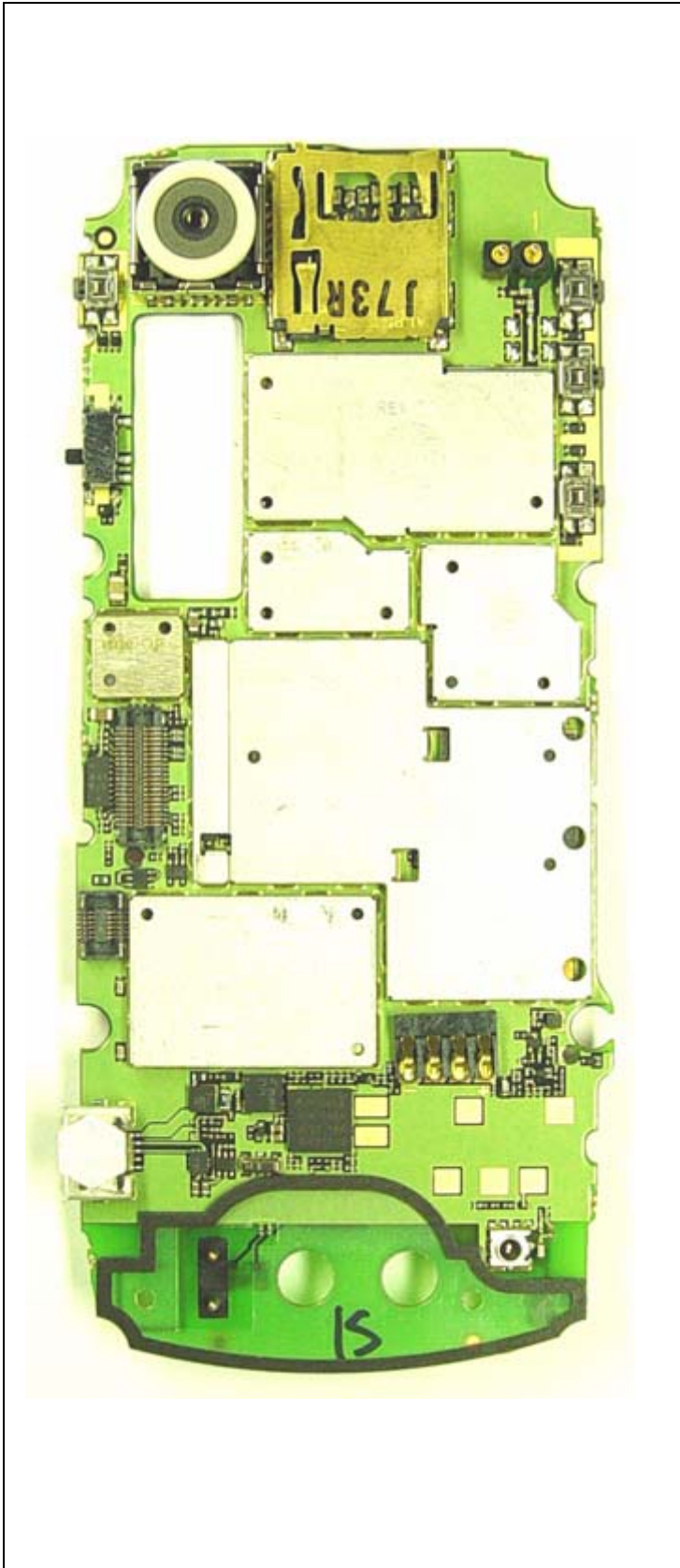
Main Board Top with Shieldcans
