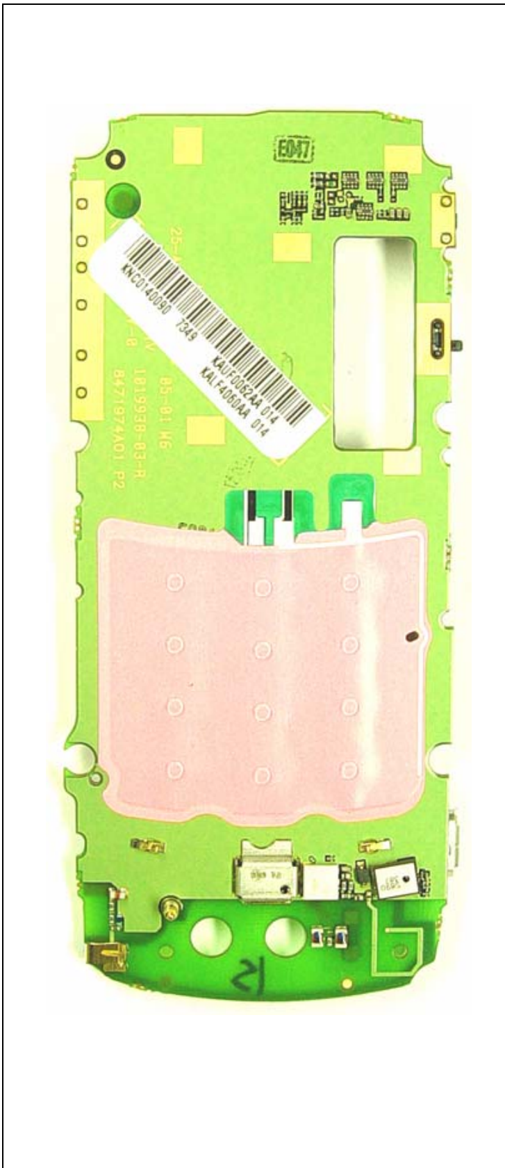
Main Board Bottom with Shieldcans and Domsheet
