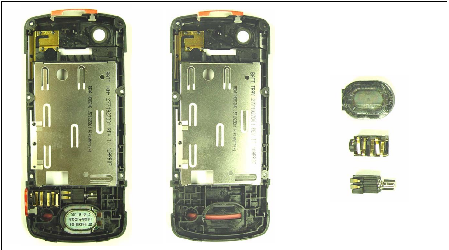
Internal Housing view of Main Rear Part
