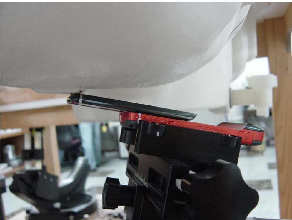
Figure 10. Phone Against the Head Phantom (15°Tilt – Slider Up)
