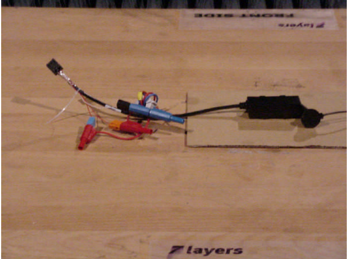
Photo 1: Setup for the "Spurious radiated emissions" up to 1GHz
