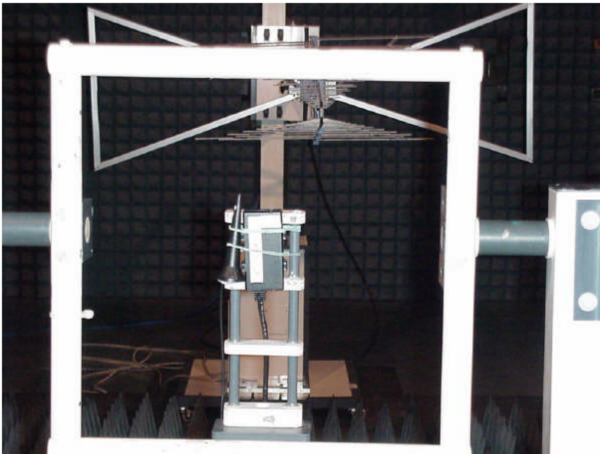
Photo 2: Setup for the "Spurious radiated emissions" above to 1GHz
