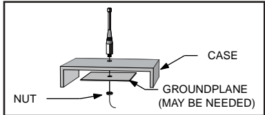
figure 18: External antenna mounting
