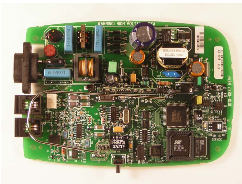
Top of the PCB
