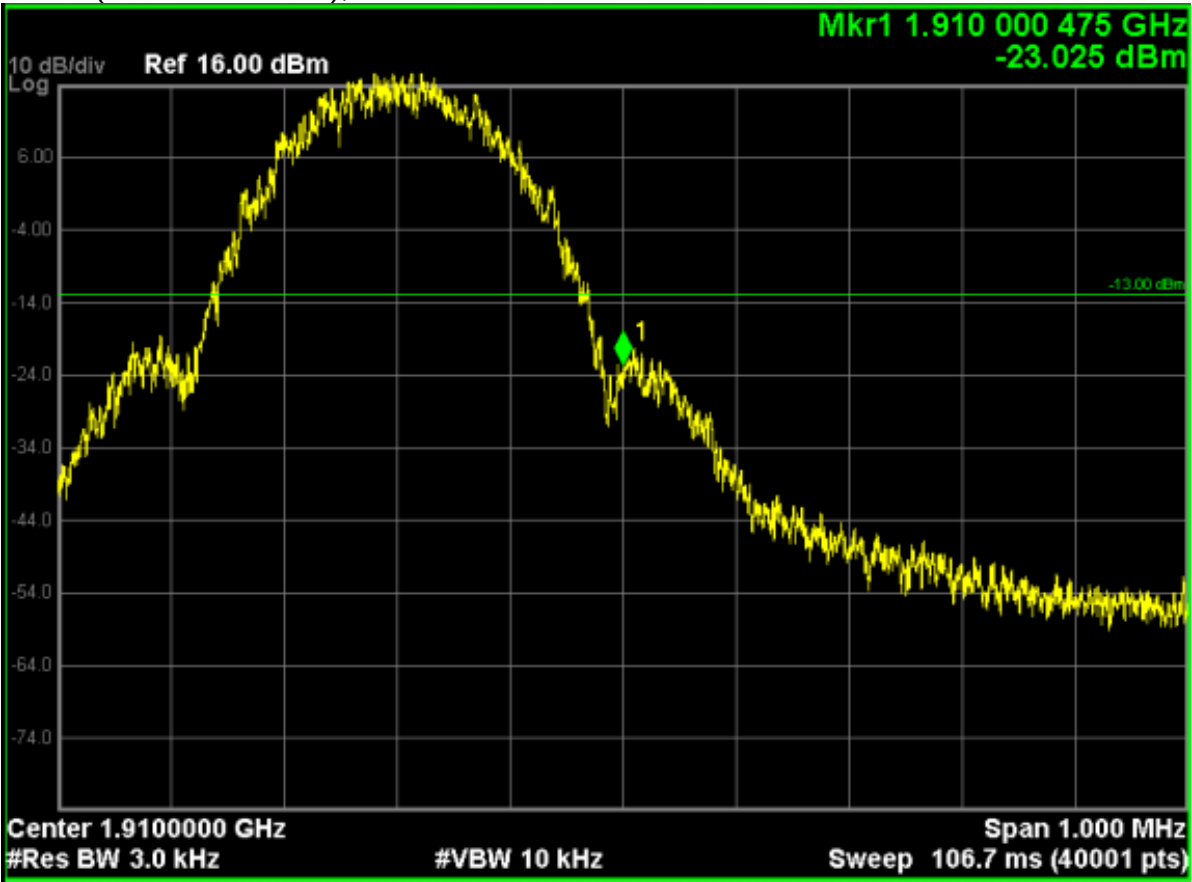
GSM1900 (EGPRS 1 Tx Slot), Channel 810
