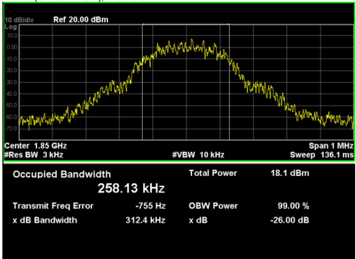
GSM1900 (GPRS 1 Tx Slot), Channel 512
