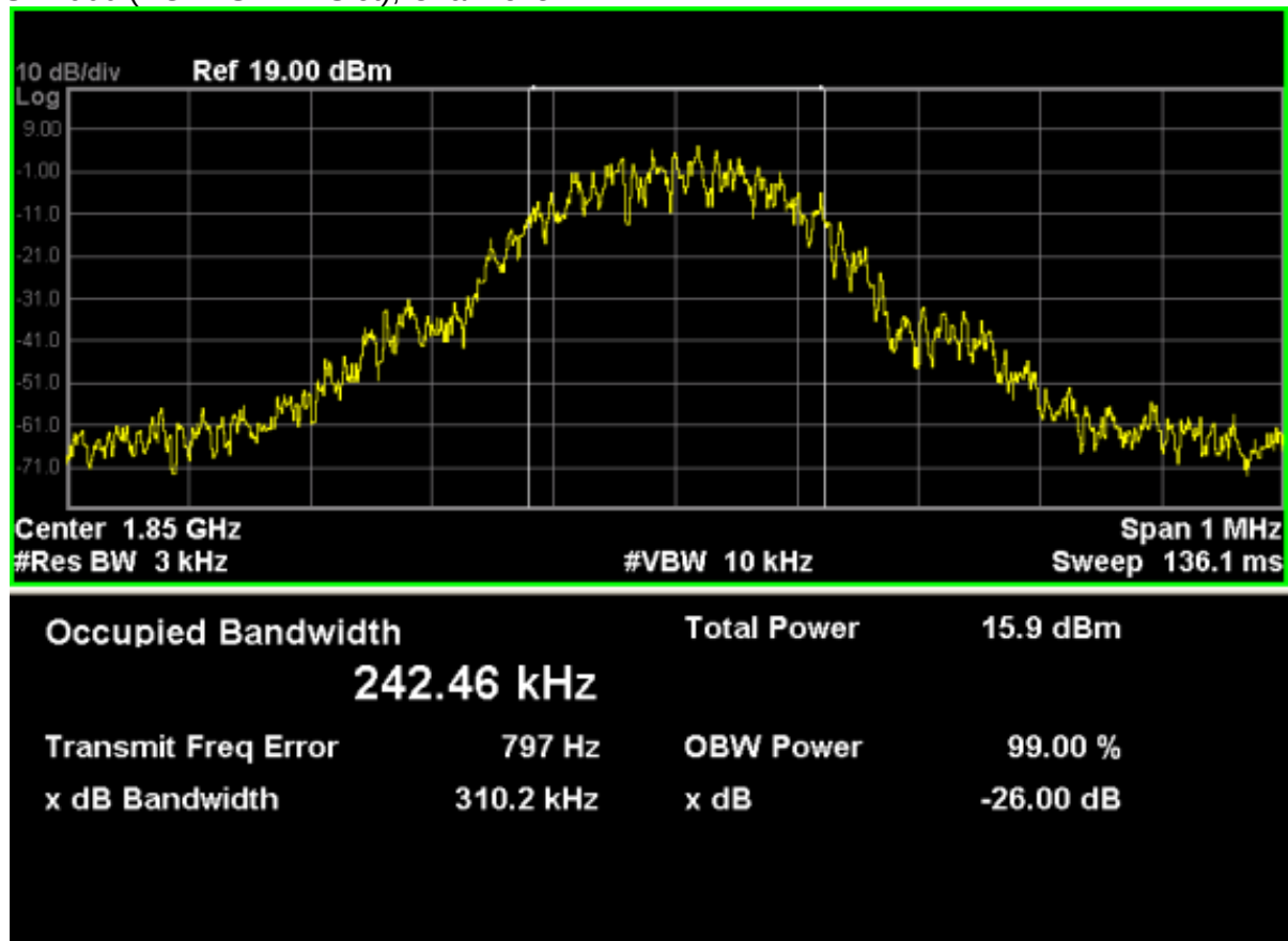
GSM1900 (EGPRS 1 Tx Slot), Channel 512
