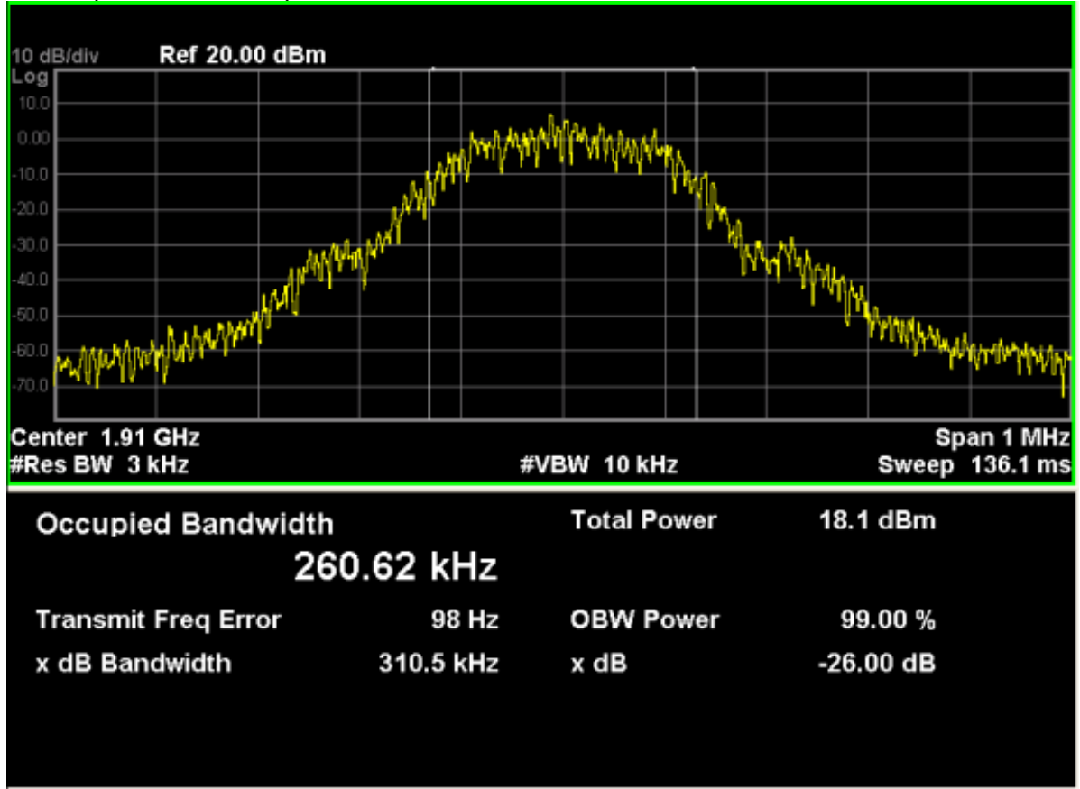
GSM1900 (GPRS 1 Tx Slot), Channel 810
