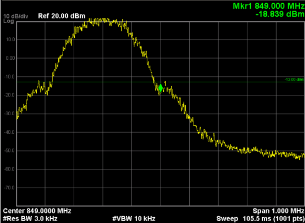
GSM850 (GPRS 1 Tx Slot), Channel 251
