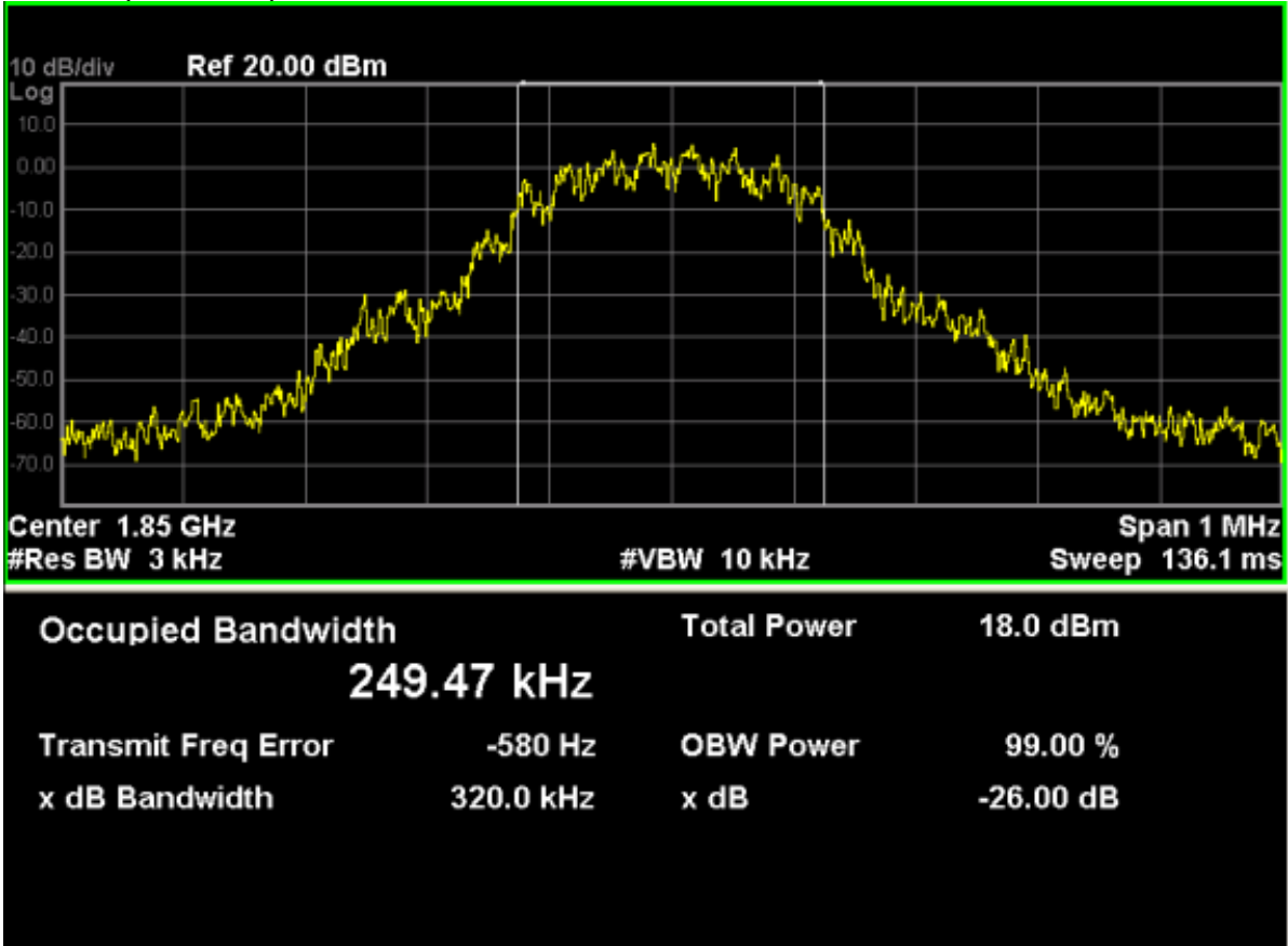
GSM1900 (GSM Link), Channel 512
