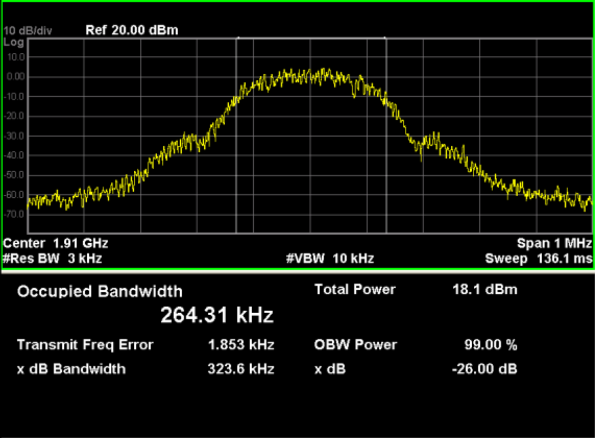
GSM1900 (GSM Link), Channel 810
