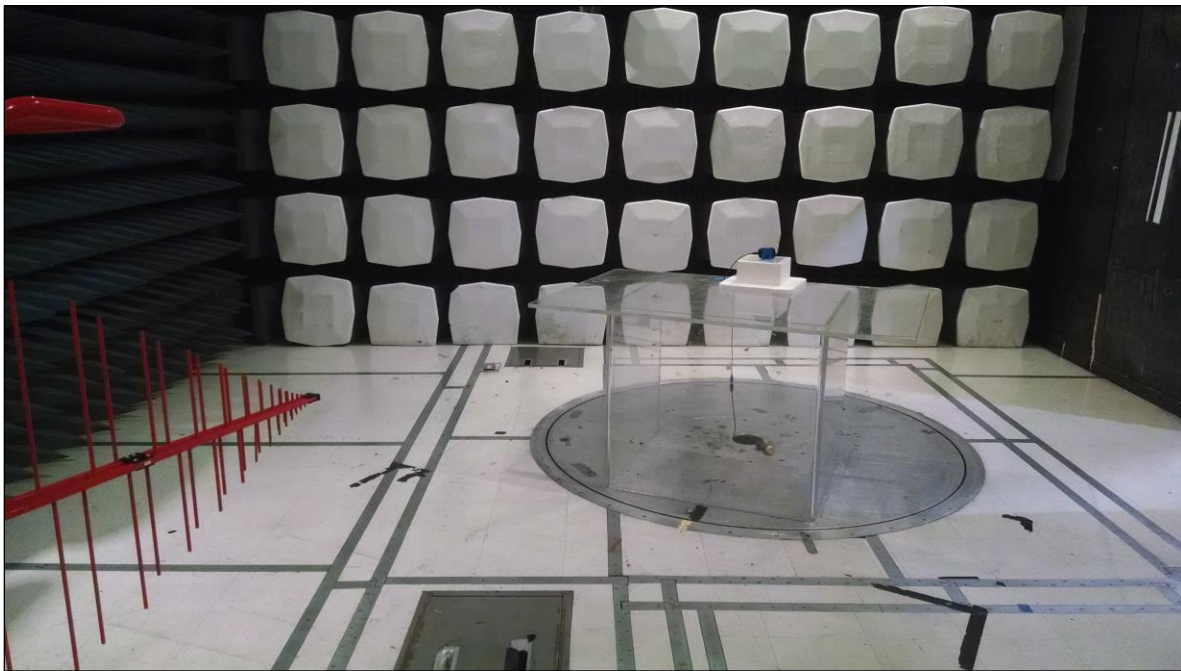
Photograph 5. Radiated Spurious Emissions below 1GHz
