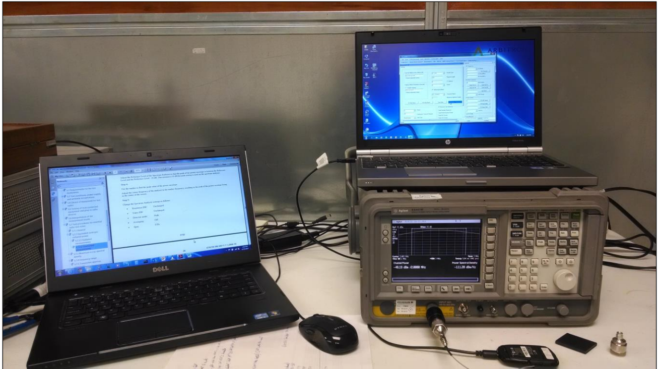
Photograph 6. Conducted Spurious Emissions, Test Setup
