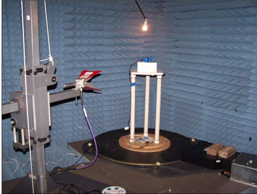
Photograph 4. Radiated Spurious Emissions above 1GHz Test Setup
