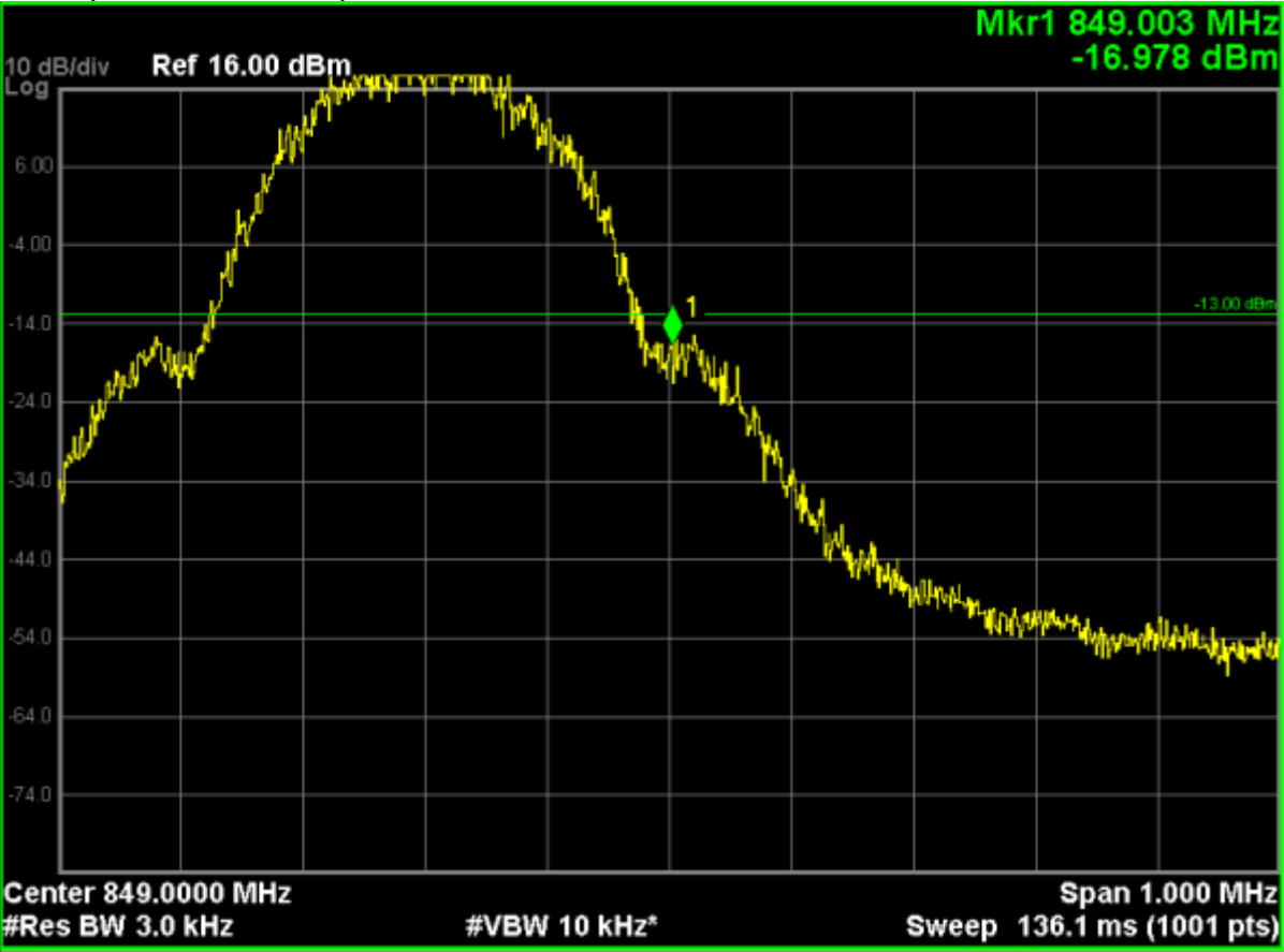
GSM850 (EGPRS 1 Tx Slot), Channel 251
