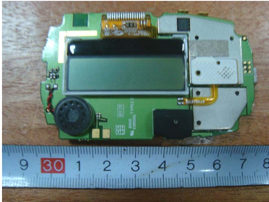
EUT – Main Board withput Shielding Bottom View
