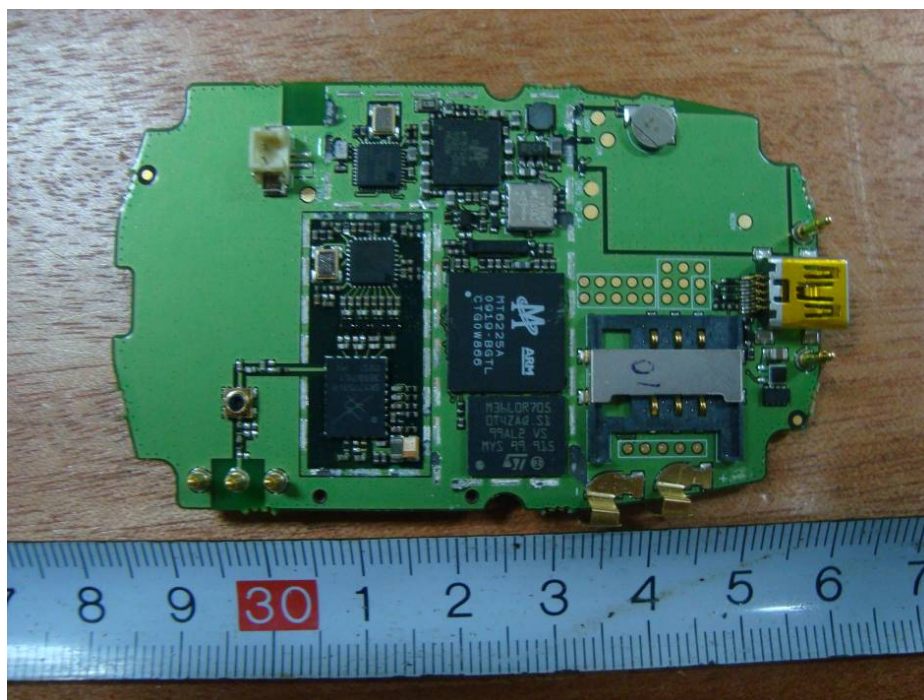
EUT –Main Board without Shielding Top View
