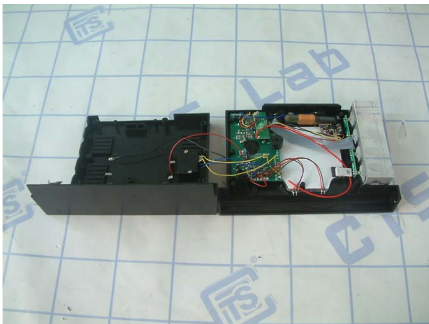
Internal view 2
