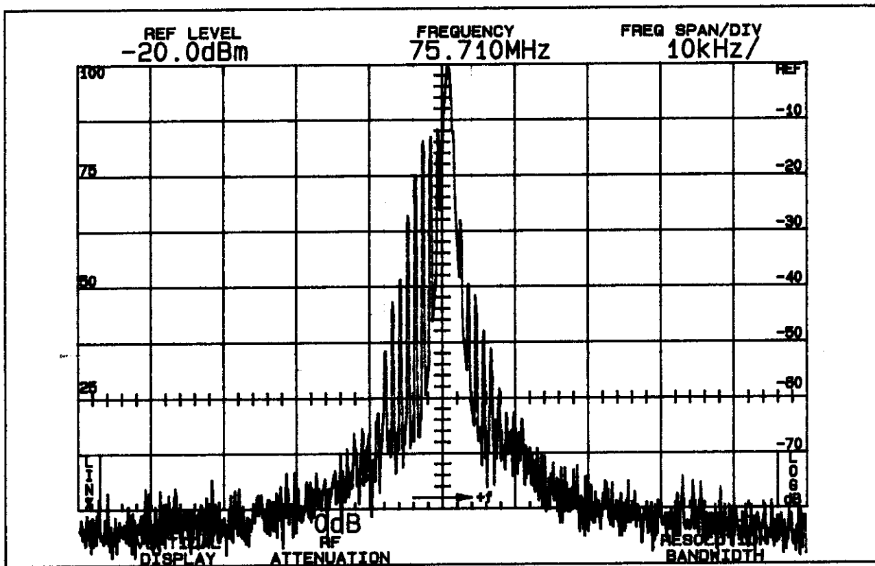
FIGURE 1 OCCUPIED BANDWIDTH
