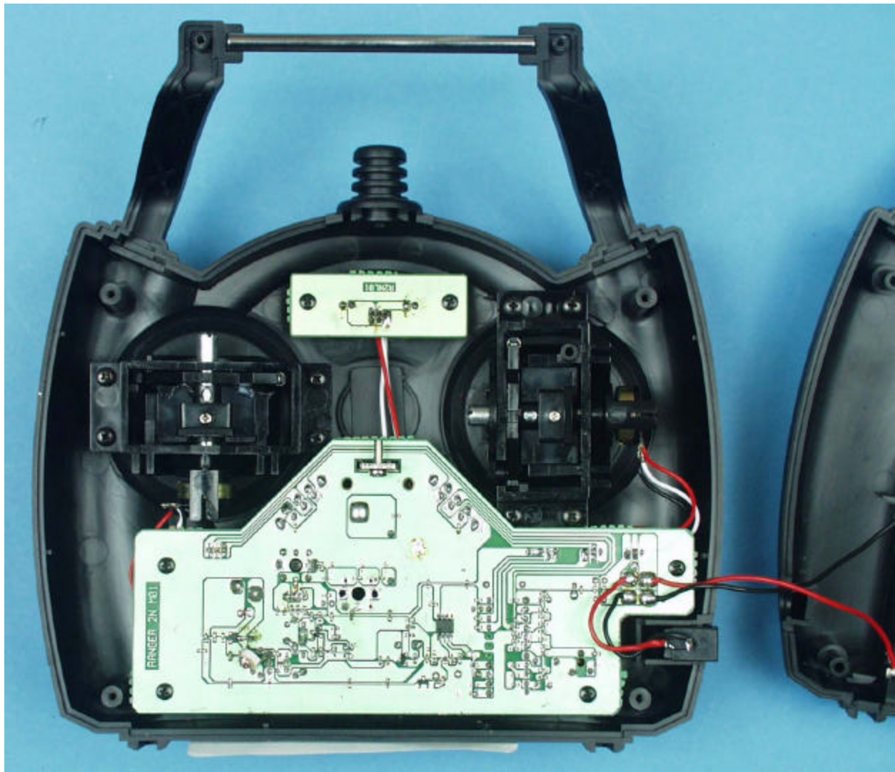
Internal, Circuit Board
