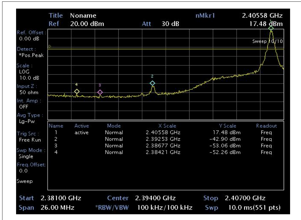
Figure 7. Plot of the Band Edge
