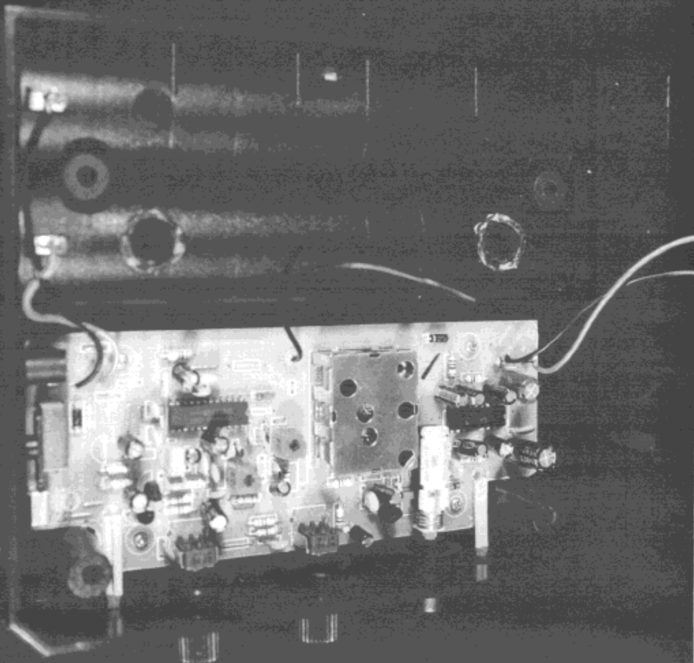
Structure View of EUT (2)
