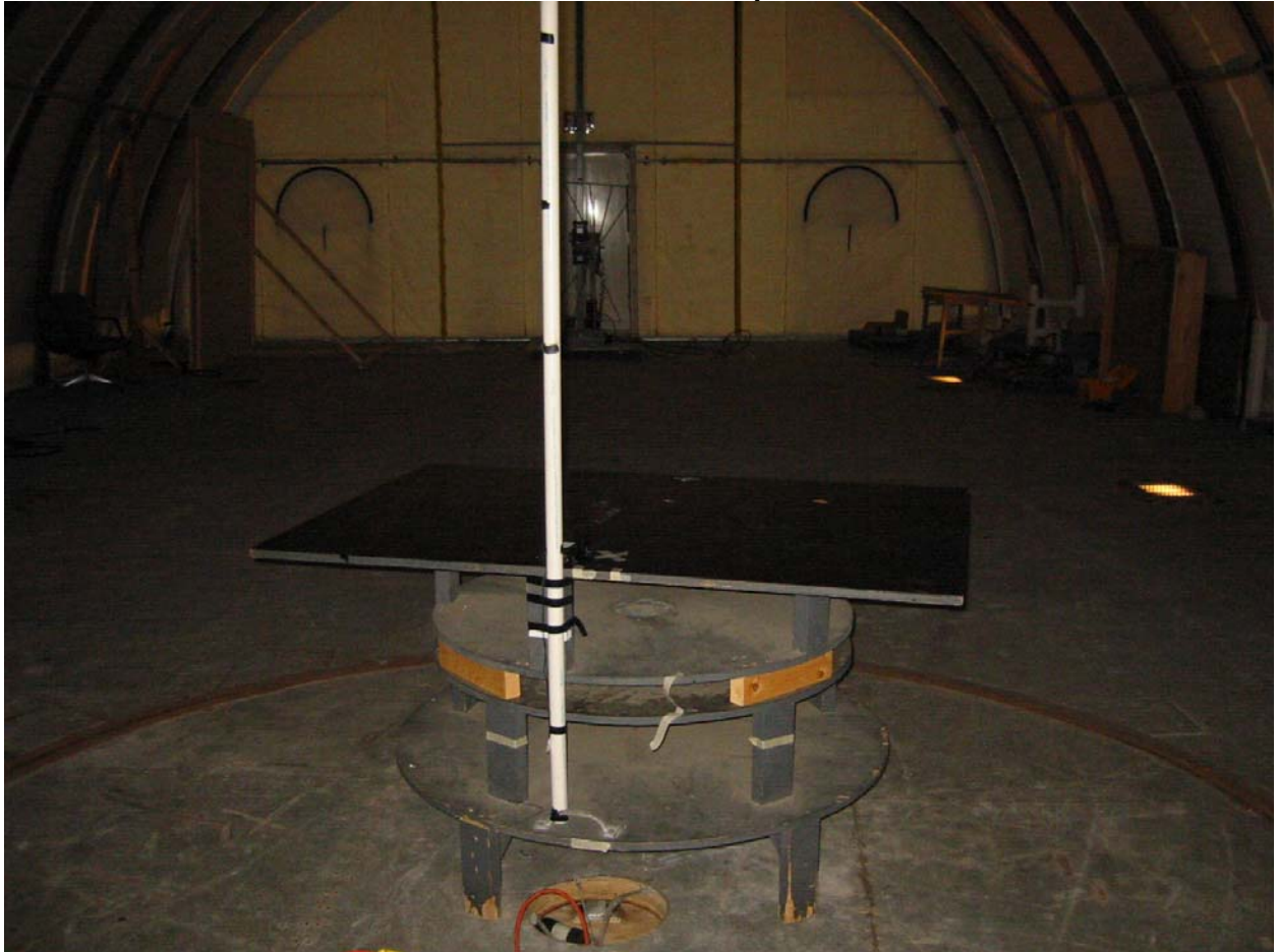
Radiated Emissions Setup Photos
