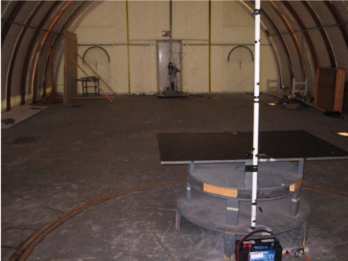
V7E-VP Part 15 30-1000 MHz
