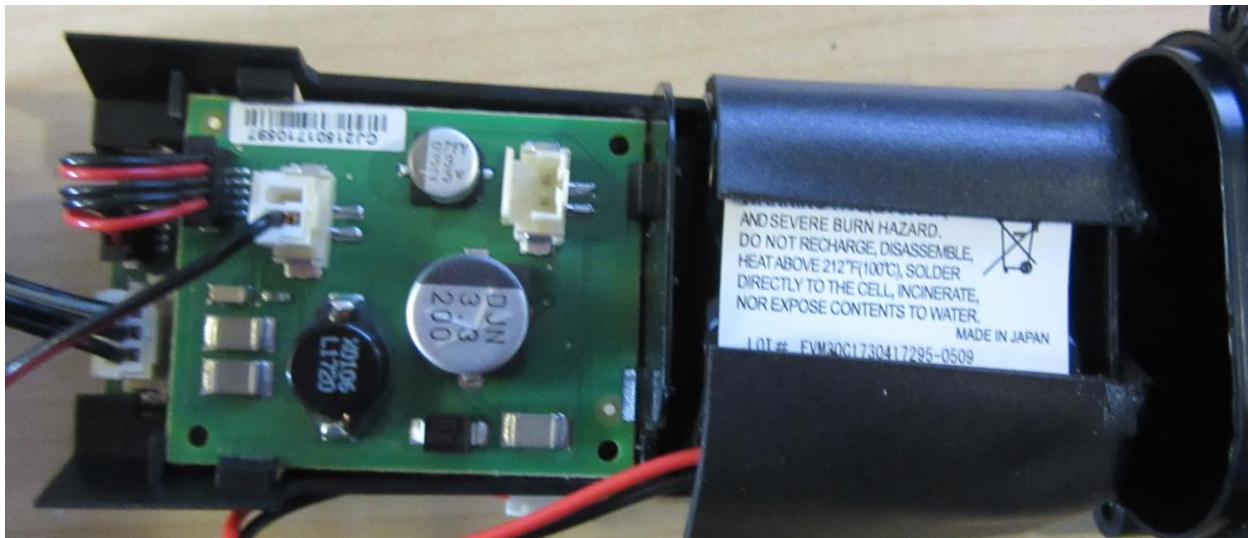
IDI-VLU10 Inside Bottom View
