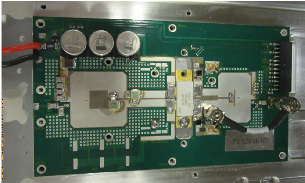
Figure 1 PA600 Power Amplifier PCB
