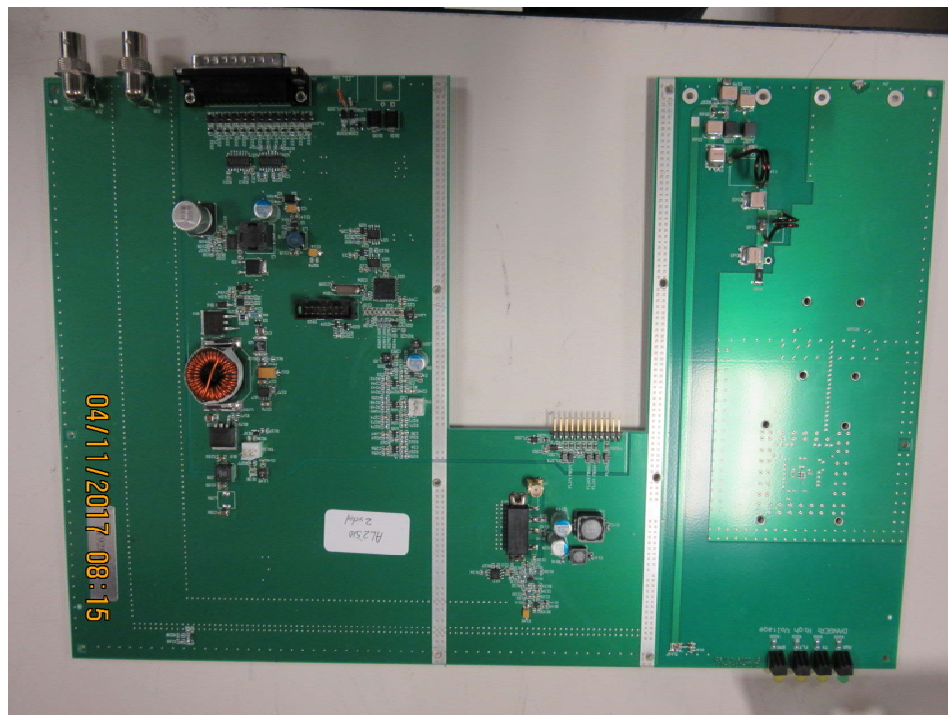
Figure 2 PA600 T/R Switch and control PCB Top
