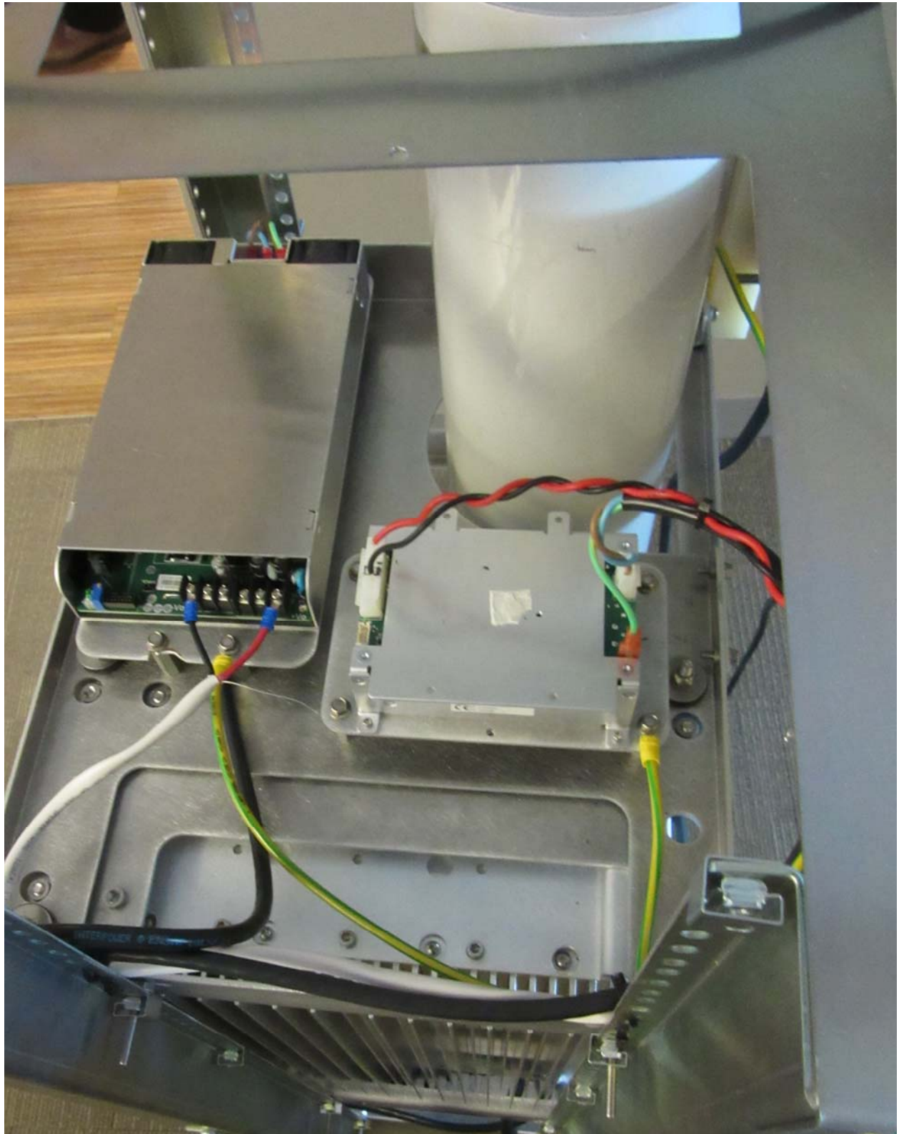
Figure 5 Top View
