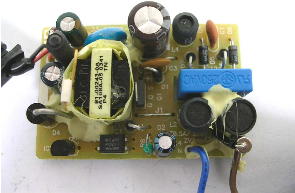
12. Rear view of PCB1
