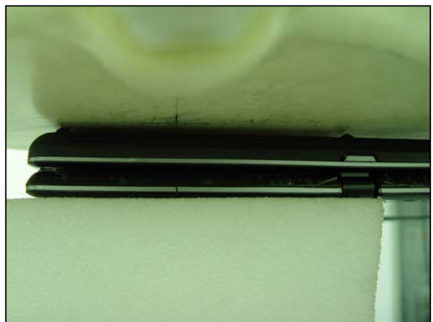
Bottom Face Touched Aux antenna
