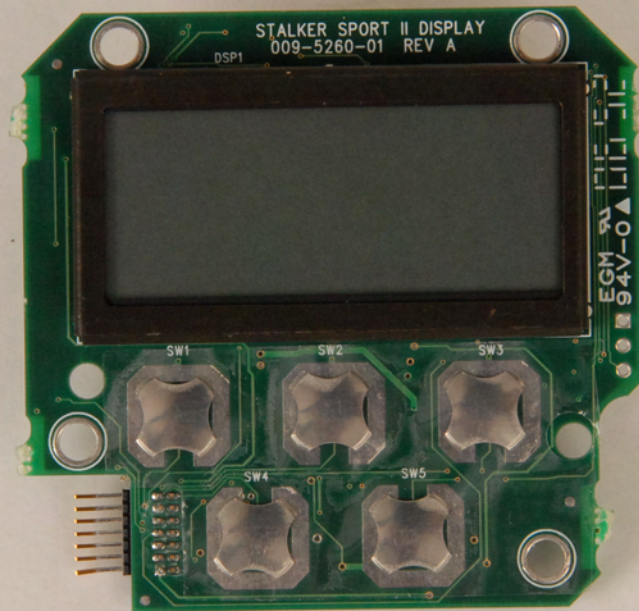
Keypad Board - Top
