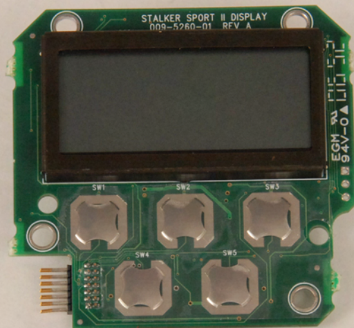
Keypad board - Top
