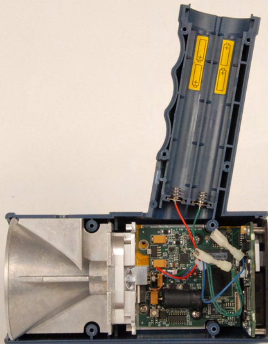
Housing Assembly - Right Side
