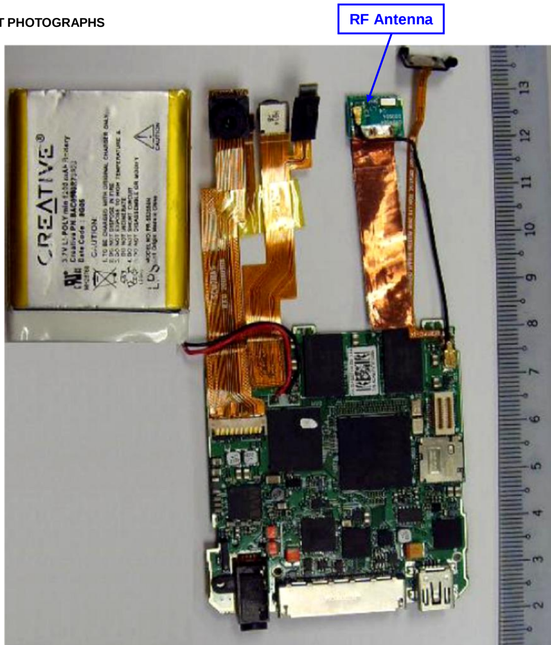
Main-Board PCB Component View
