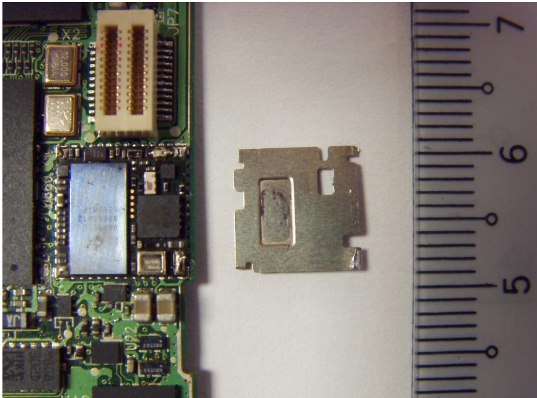
RF Module Circuit with RF Shield Removed
