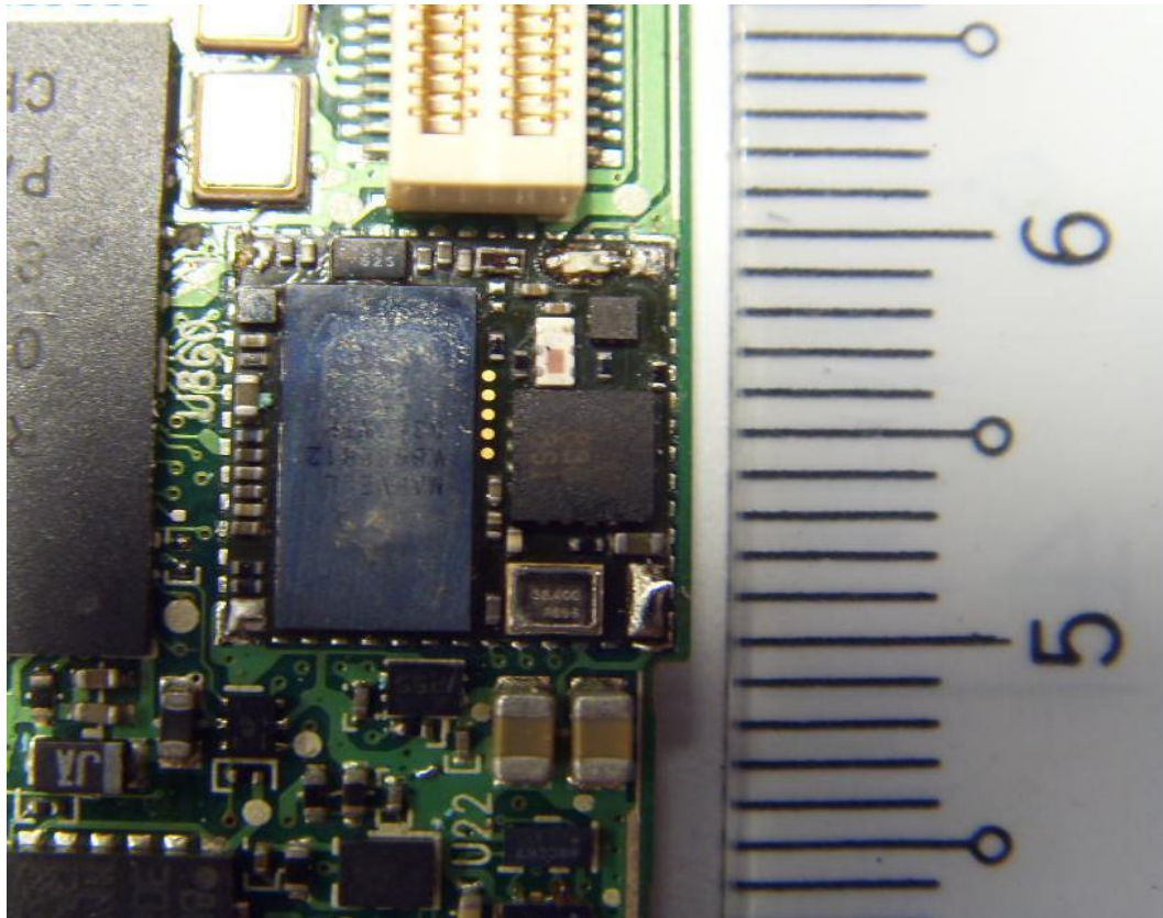
Close View of RF Module Circuit with RF Shield Removed
