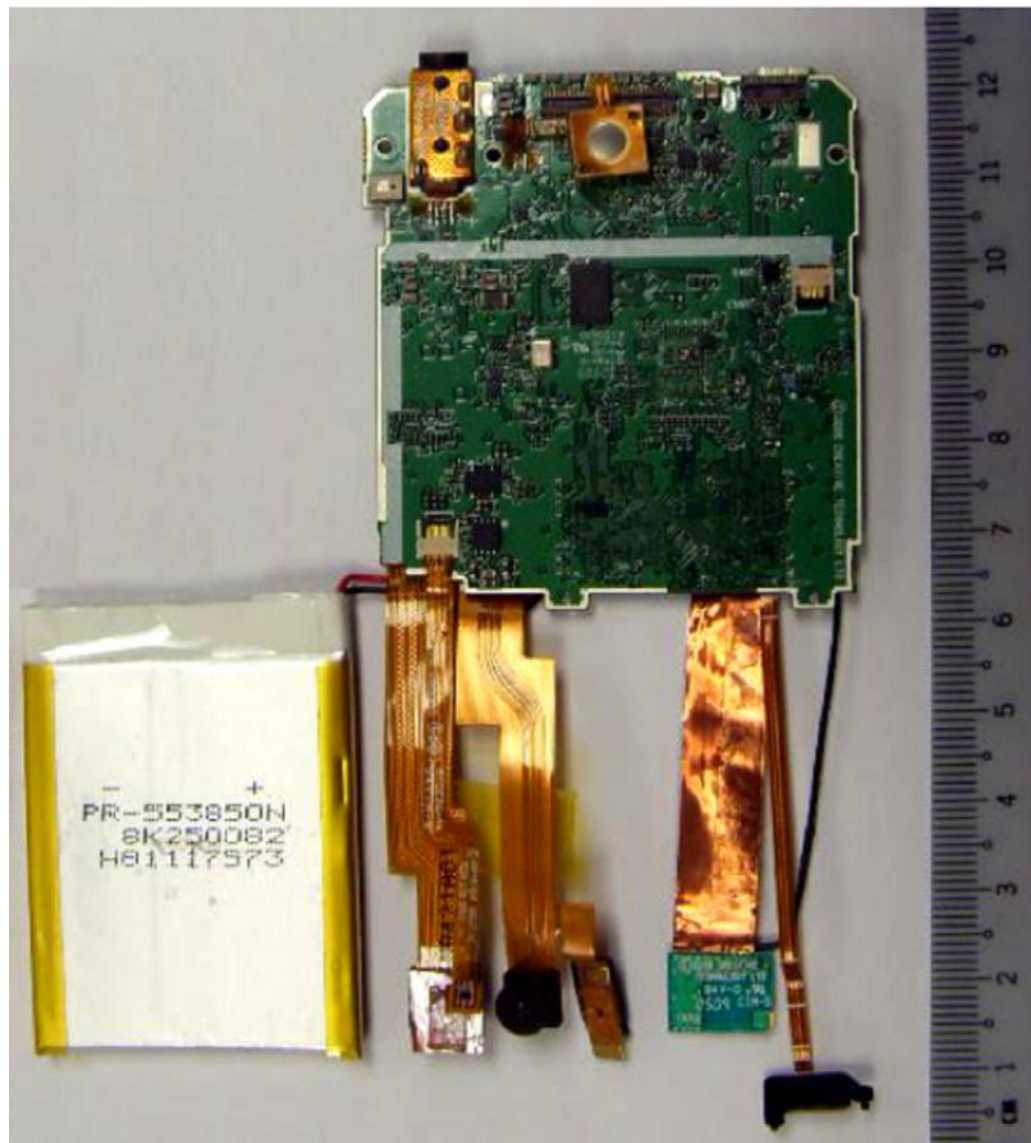
Main-Board PCB Trace View
