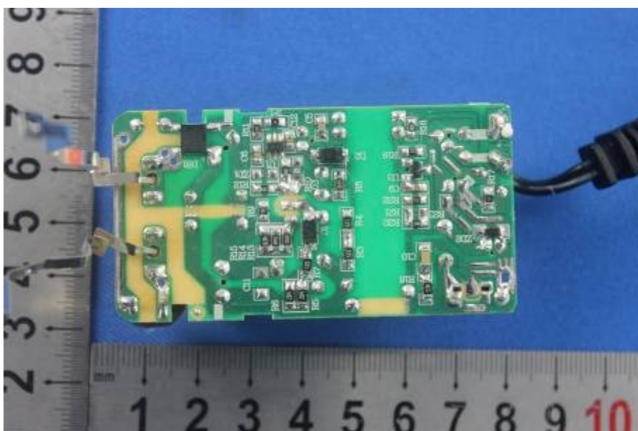
Power supply unit (model No.: GPE125-130100-Z)
