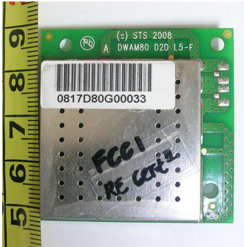
RF Module Circuit – Component Side with RF Shield
