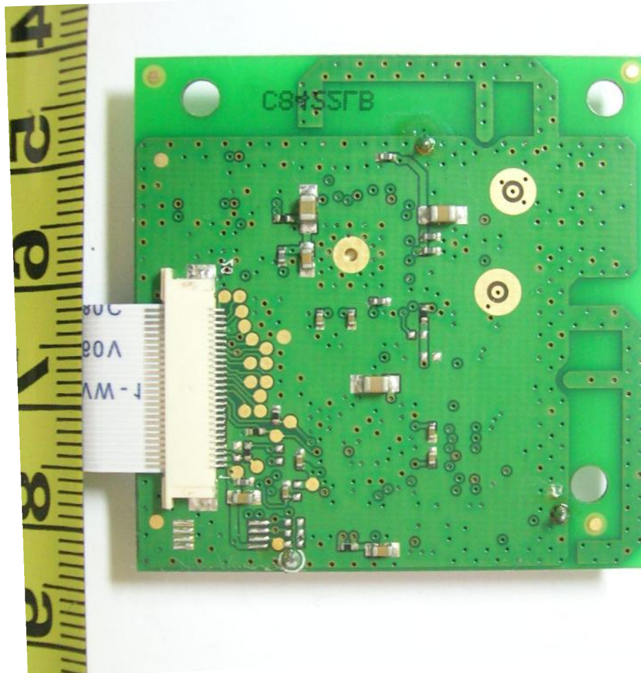
RF Module Circuit Trace Side
