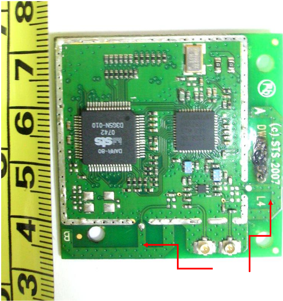
RF Module Circuit – Component Side with RF Shield Removed
