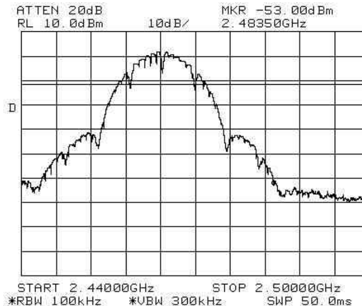
Plot 16 – Upper Band Edge at 2.4835GHz
