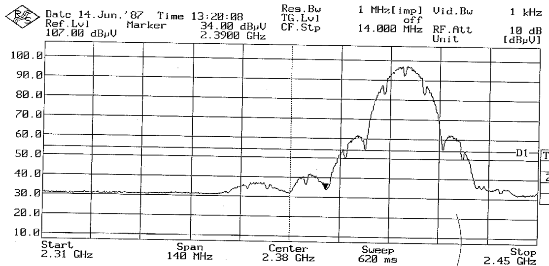
Plot 20 – Average Plot at Lower Band Edge at 2.4000GHz
