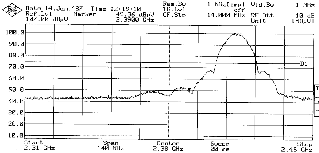
Plot 19 – Peak Plot at Lower Band Edge at 2.4000GHz
