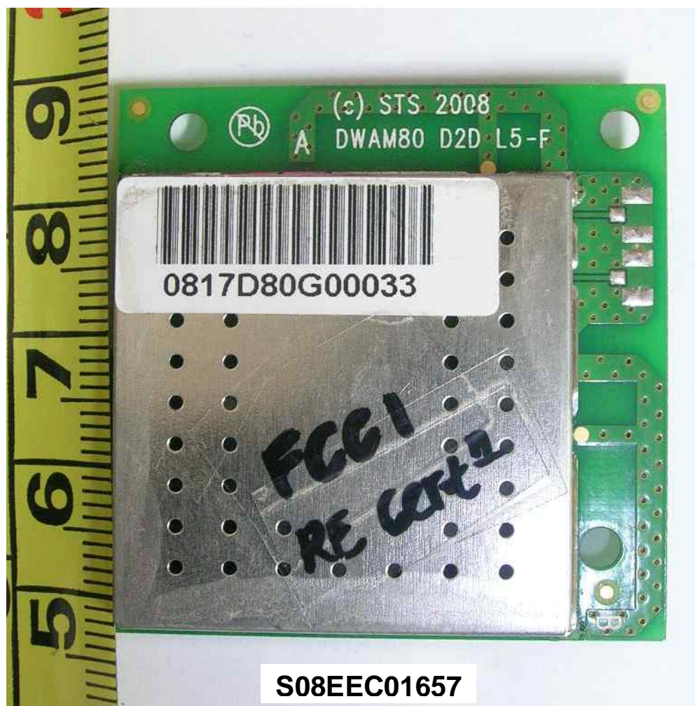
S08EEC01657 RF Module Circuit – Component Side with RF Shield
