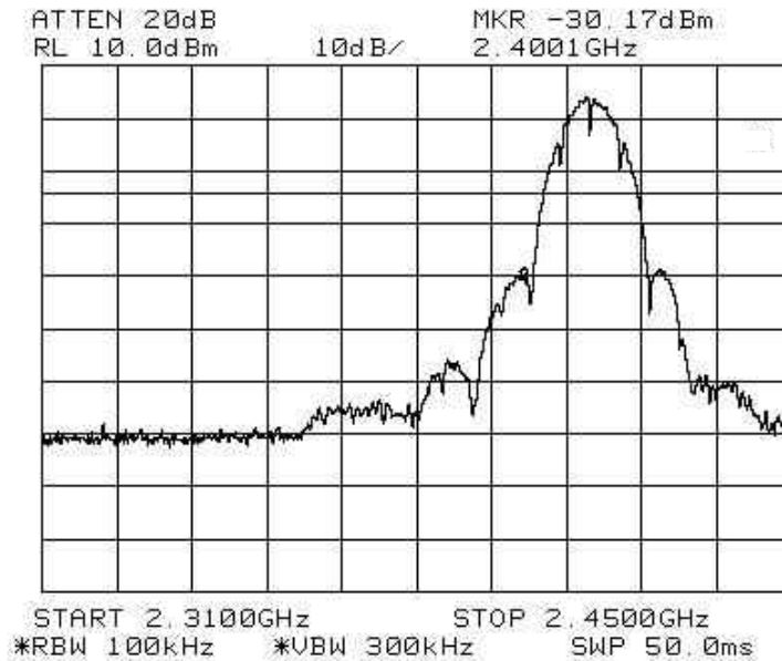
Plot 15 – Lower Band Edge at 2.4000GHz
