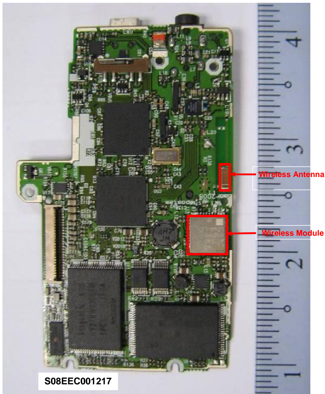
RF Module Circuit with RF Shield
