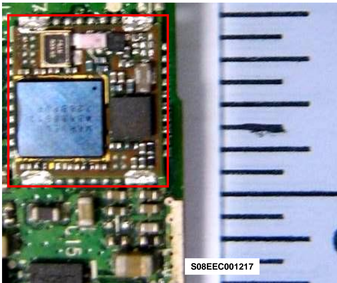
RF Module Circuit with RF Shield Removed
