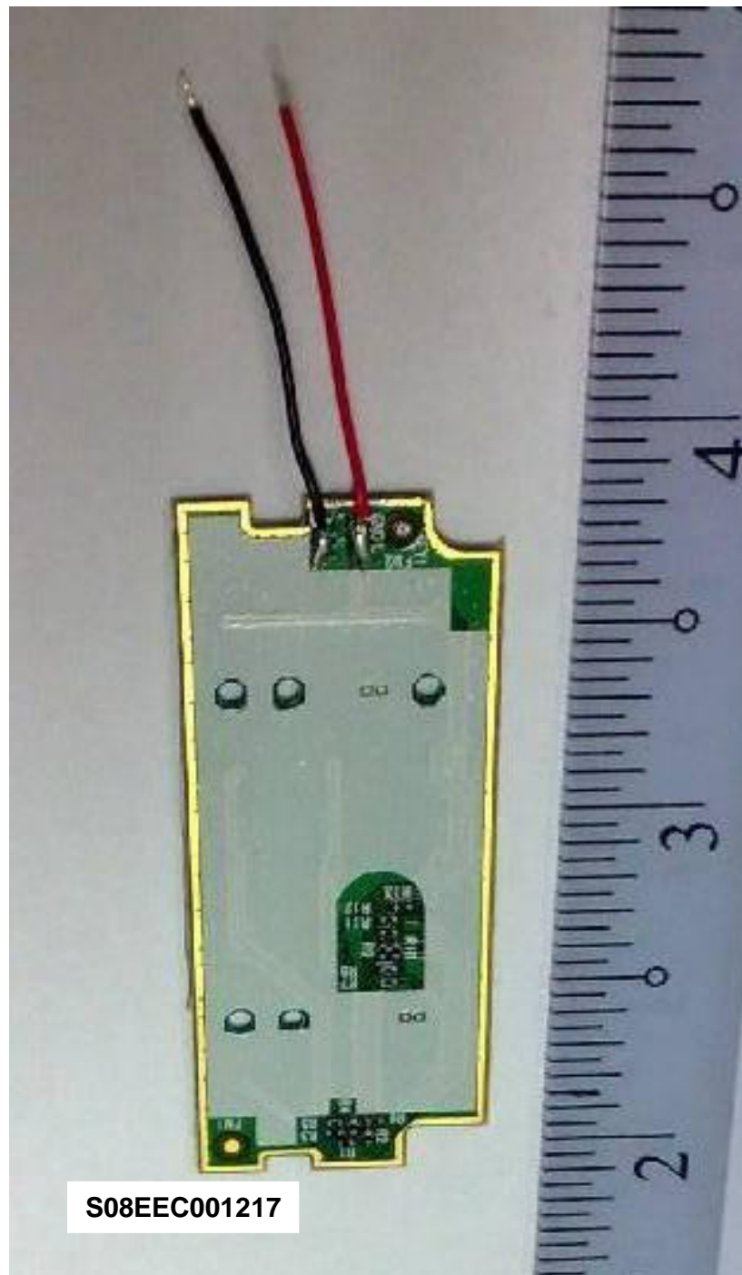
Keypad Trace Side
