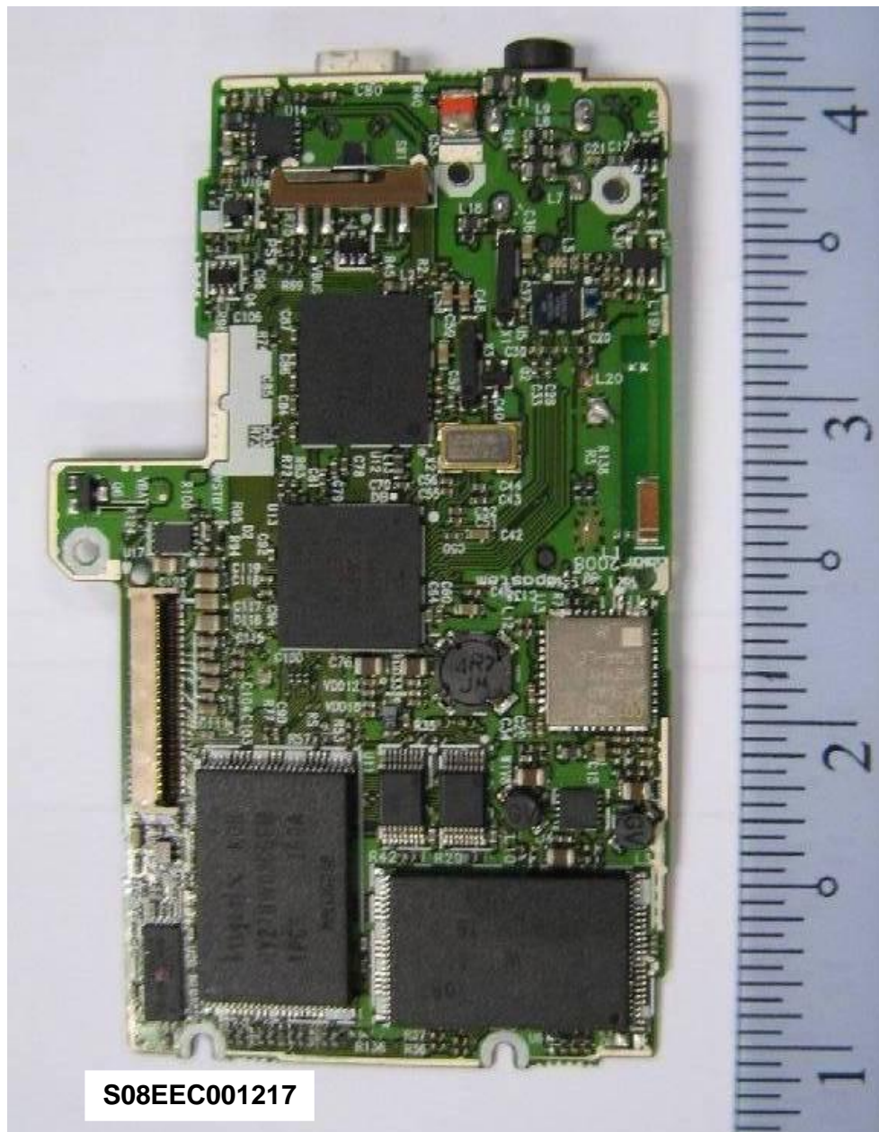
Main Board - View 2
