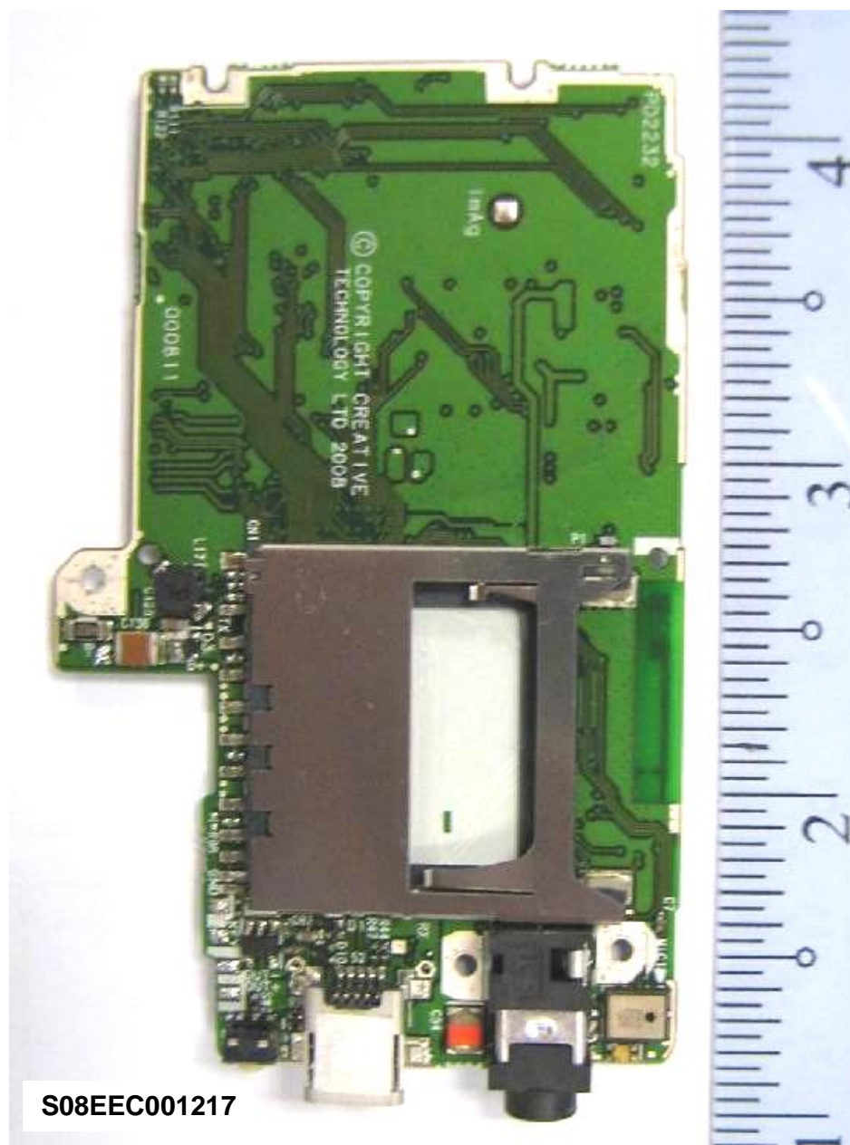
Main Board – View 1
