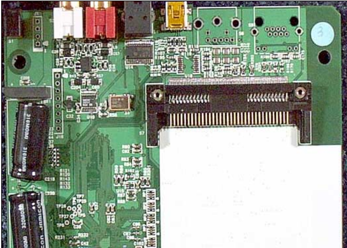
Base Top Digital Card Close up 1
