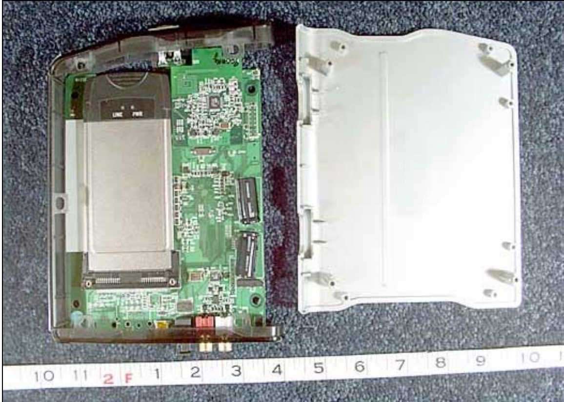
Base Bottom Cover Removed
