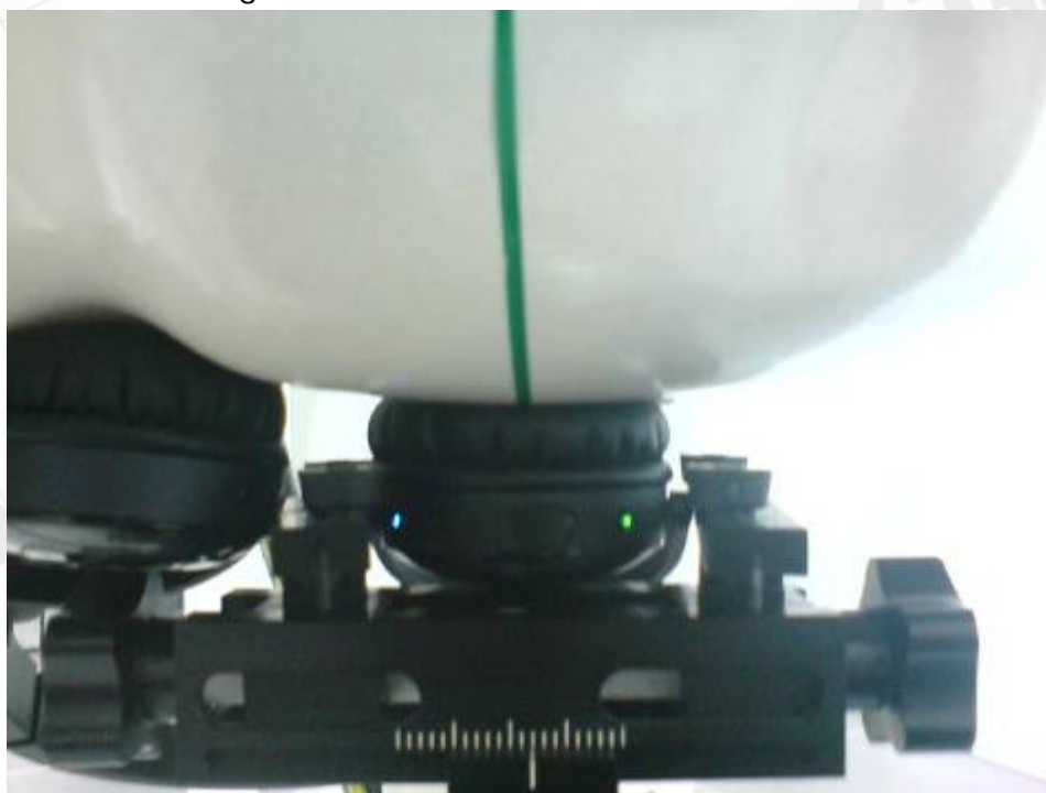
Fig.3.2 Left Head Section / Cheek-Touch Position
