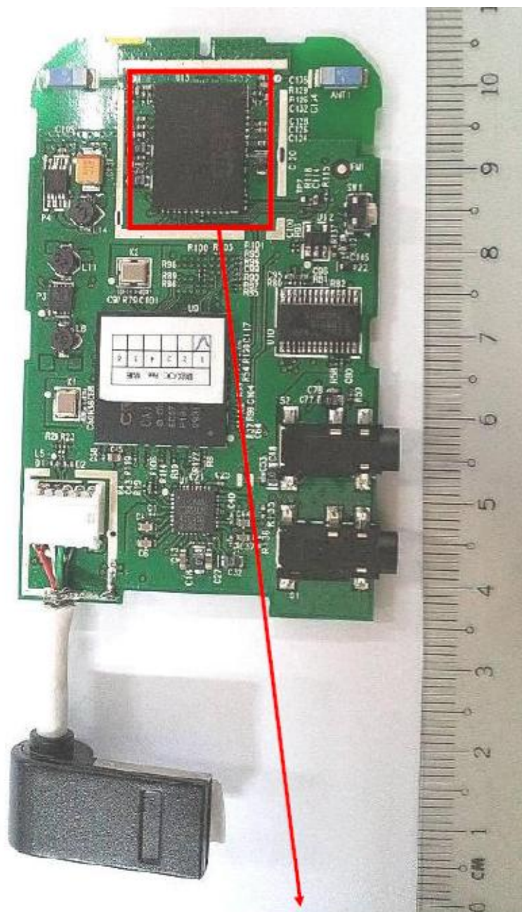
RF Module Circuit with RF Shield Removed
