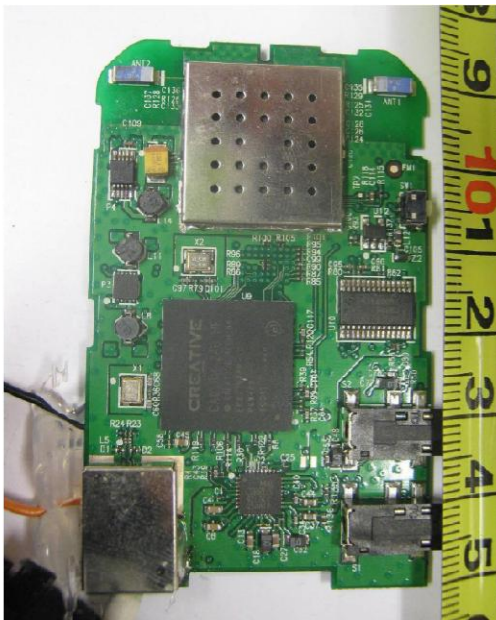
Main-Board PCB Component Side
