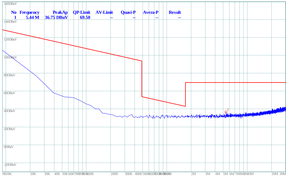
(Plot B.0: 9kHz to 30MHz @ 11/4-DQPSK, channel 39)
