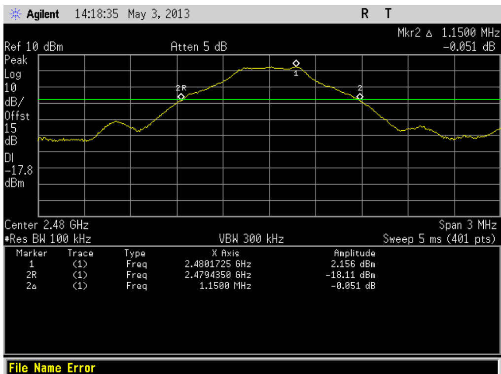
(Plot C1: Channel = 2480 @ GFSK)
