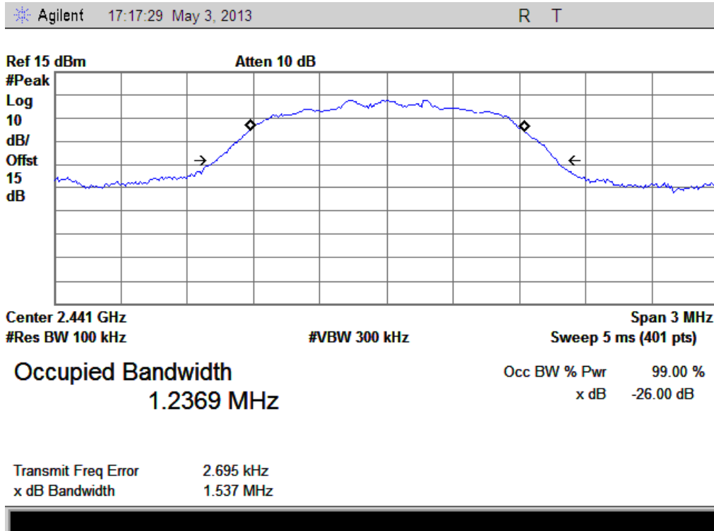
(Plot E2: Channel = 2441 @ \pi/4 -DQPSK)
