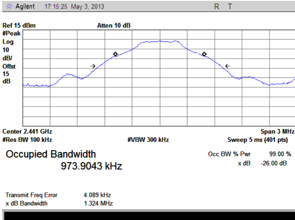
(Plot B2: Channel = 2441 @ GFSK)
