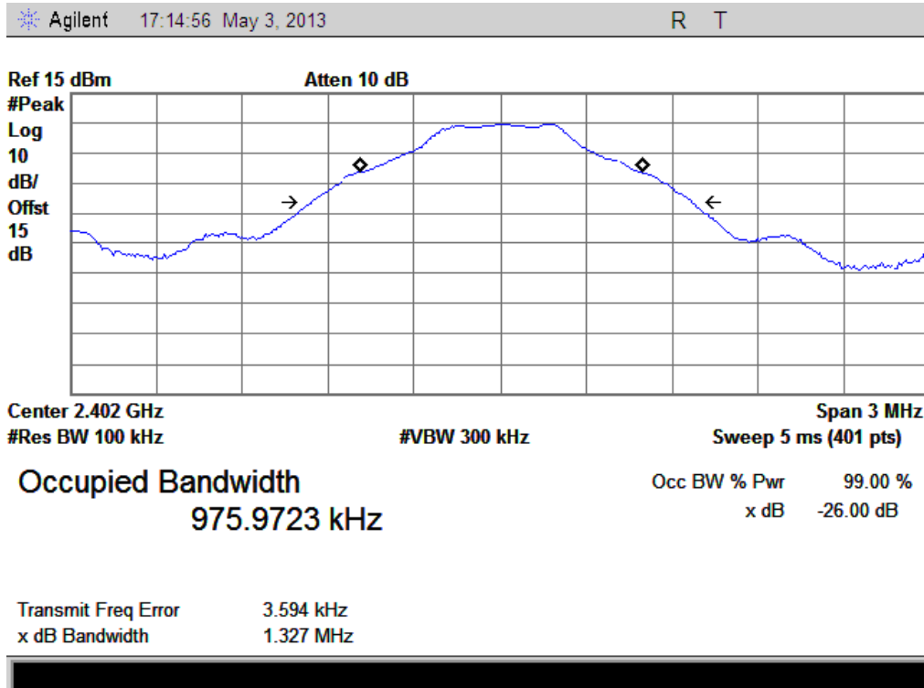
(Plot A2: Channel = 2402 @ GFSK)
