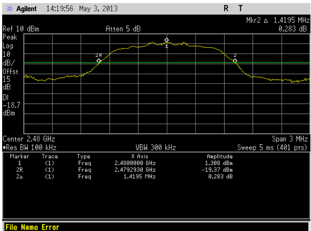
(Plot F1: Channel = 2480 @ \pi/4 -DQPSK)
