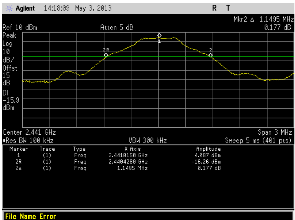
(Plot B1: Channel = 2441 @ GFSK)
